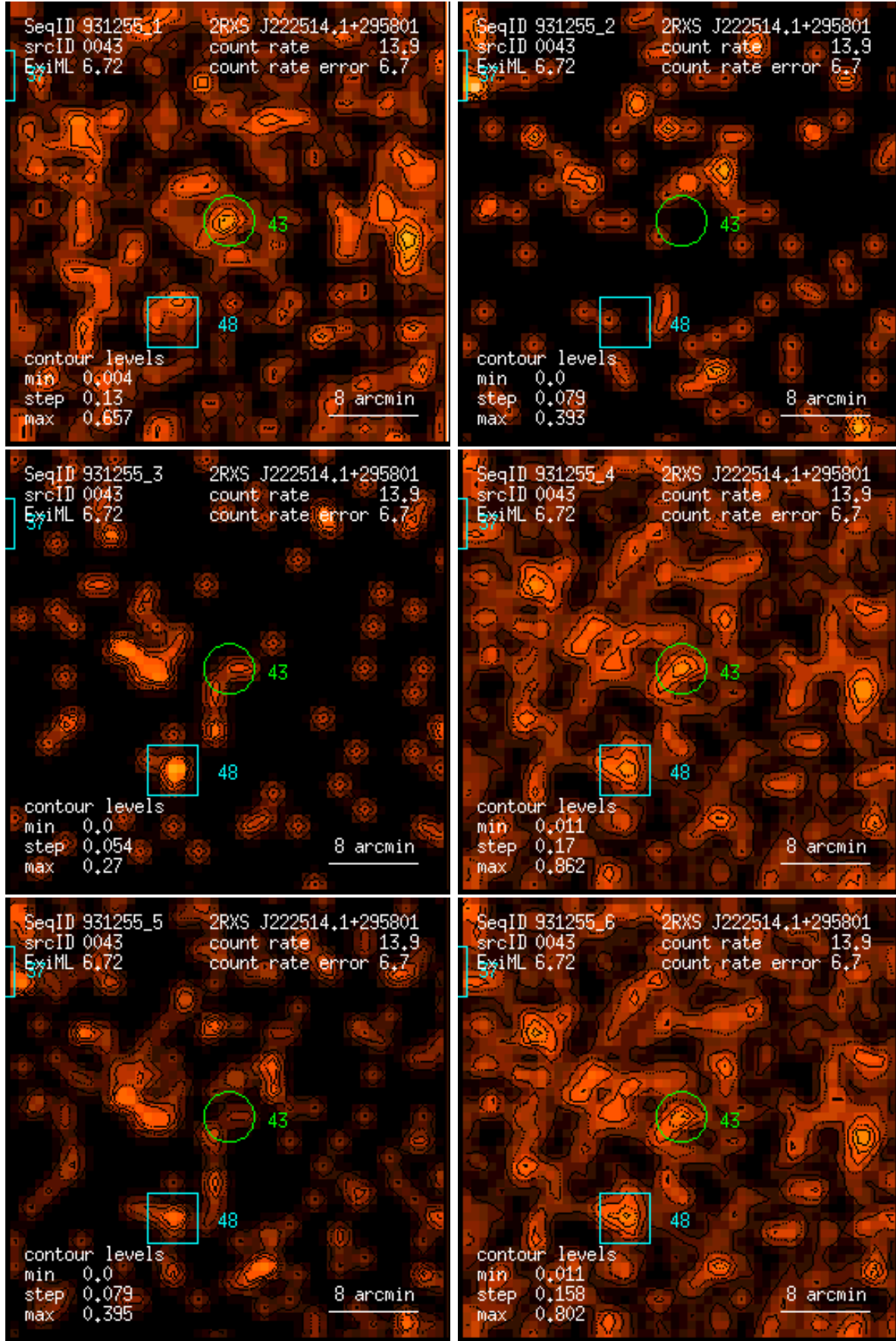
Figure 43: RASS 931255: detection 0043: band rate images, Gaussian filter: (1) PSPC channels 11 – 41, (2) 52 – 90, (3) 91 – 201, (4) 11 – 235, (5) 52 – 201, (6) 11 – 201. Broad band rates in counts/ks. Band rate contour levels in counts/ks/arcmin 2 .
