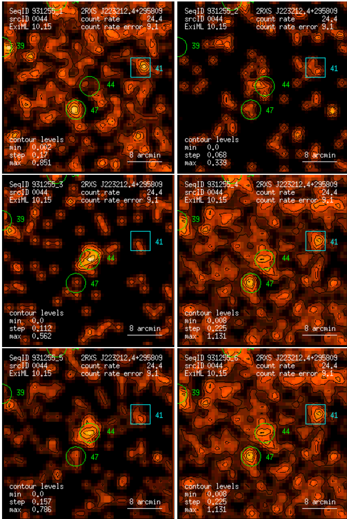
Figure 44: RASS 931255: detection 0044: band rate images, Gaussian filter: (1) PSPC channels 11 – 41, (2) 52 – 90, (3) 91 – 201, (4) 11 – 235, (5) 52 – 201, (6) 11 – 201. Broad band rates in counts/ks. Band rate contour levels in counts/ks/arcmin 2 .
