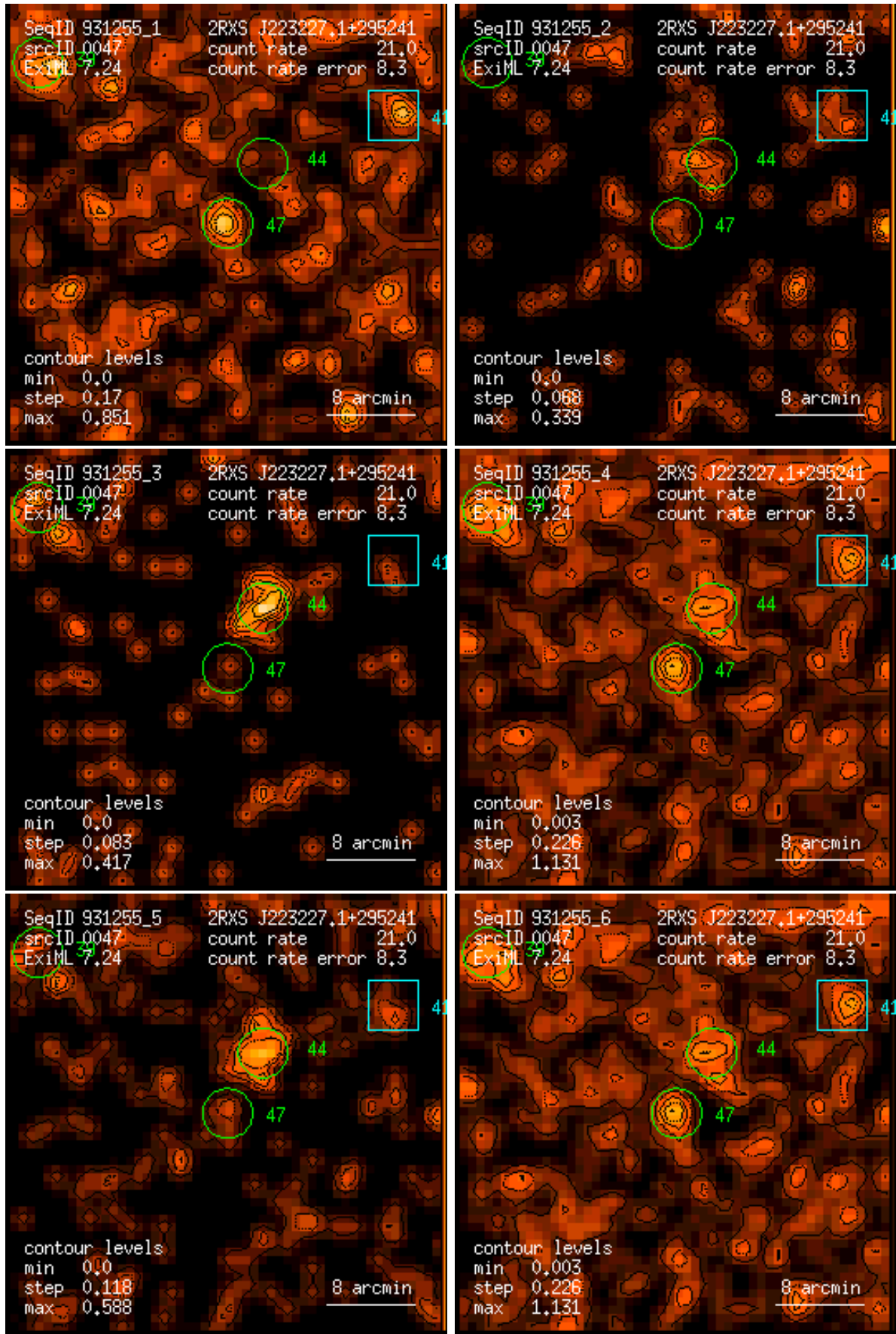
Figure 47: RASS 931255: detection 0047: band rate images, Gaussian filter: (1) PSPC channels 11 – 41, (2) 52 – 90, (3) 91 – 201, (4) 11 – 235, (5) 52 – 201, (6) 11 – 201. Broad band rates in counts/ks. Band rate contour levels in counts/ks/arcmin 2 .
