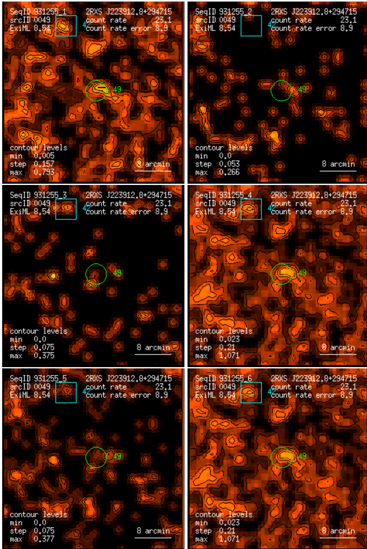
Figure 49: RASS 931255: detection 0049: band rate images, Gaussian filter: (1) PSPC channels 11 – 41, (2) 52 – 90, (3) 91 – 201, (4) 11 – 235, (5) 52 – 201, (6) 11 – 201. Broad band rates in counts/ks. Band rate contour levels in counts/ks/arcmin 2 .
