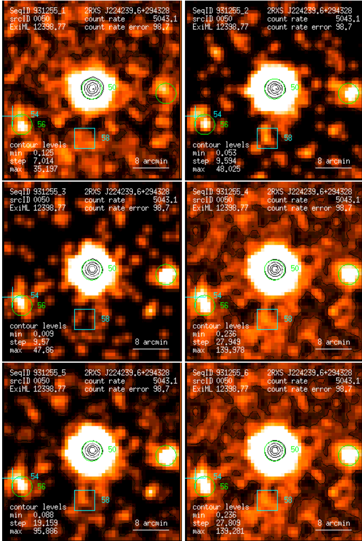
Figure 50: RASS 931255: detection 0050: band rate images, Gaussian filter: (1) PSPC channels 11 – 41, (2) 52 – 90, (3) 91 – 201, (4) 11 – 235, (5) 52 – 201, (6) 11 – 201. Broad band rates in counts/ks. Band rate contour levels in counts/ks/arcmin 2 .
