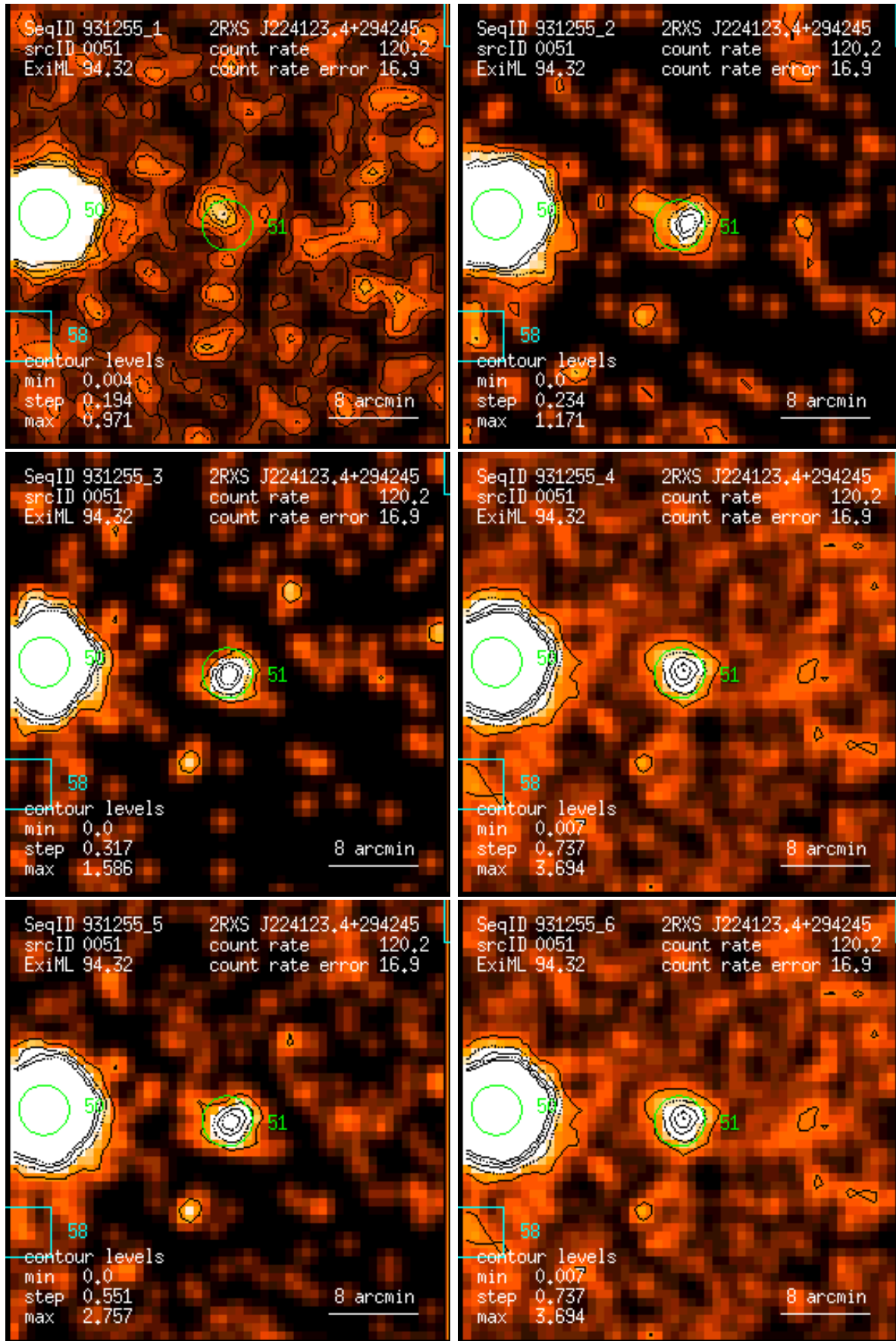
Figure 51: RASS 931255: detection 0051: band rate images, Gaussian filter: (1) PSPC channels 11 – 41, (2) 52 – 90, (3) 91 – 201, (4) 11 – 235, (5) 52 – 201, (6) 11 – 201. Broad band rates in counts/ks. Band rate contour levels in counts/ks/arcmin 2 .
