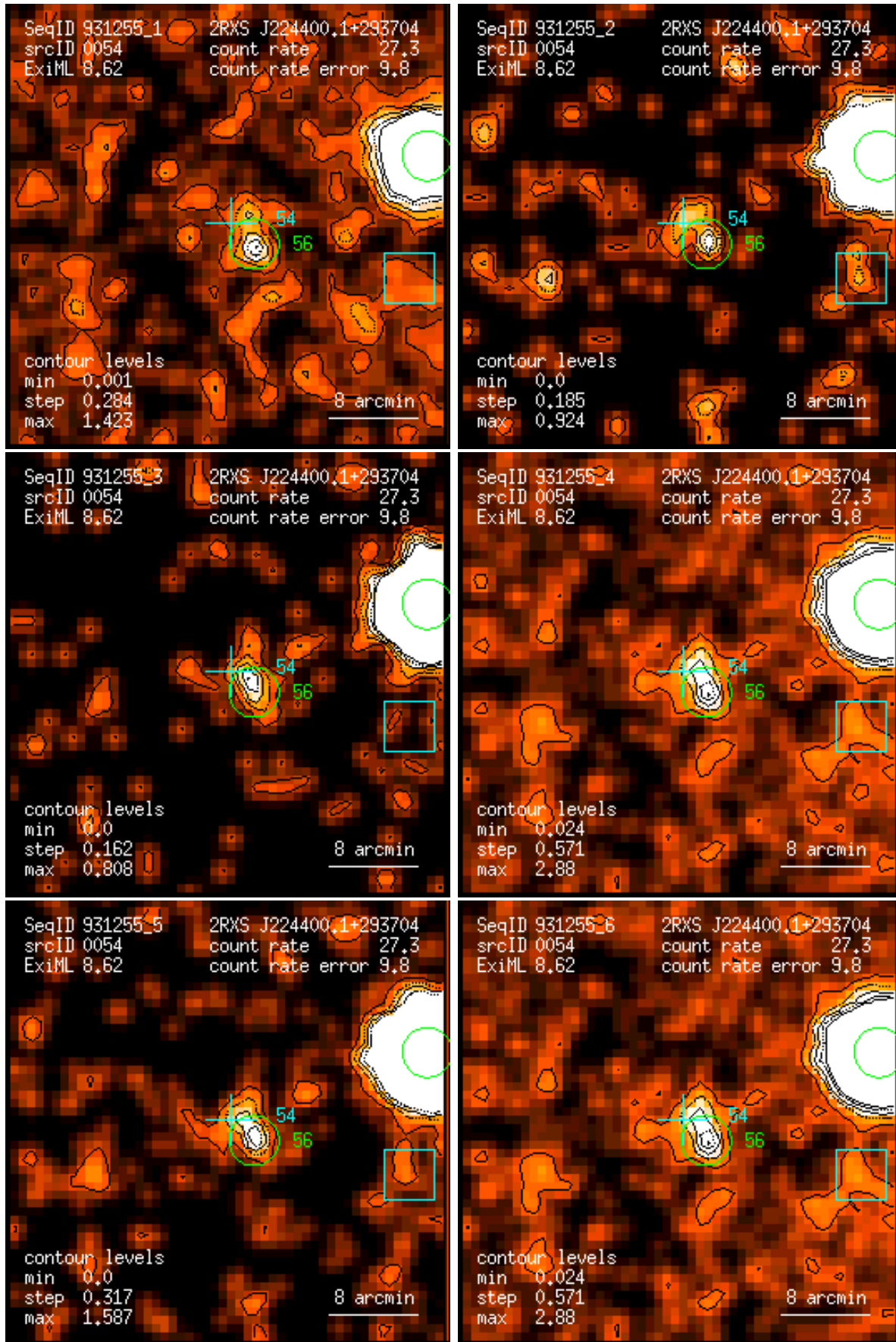
Figure 54: RASS 931255: detection 0054: band rate images, Gaussian filter: (1) PSPC channels 11 – 41, (2) 52 – 90, (3) 91 – 201, (4) 11 – 235, (5) 52 – 201, (6) 11 – 201. Broad band rates in counts/ks. Band rate contour levels in counts/ks/arcmin 2 .
