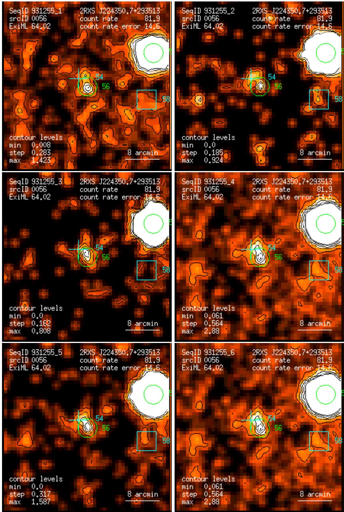
Figure 56: RASS 931255: detection 0056: band rate images, Gaussian filter: (1) PSPC channels 11 – 41, (2) 52 – 90, (3) 91 – 201, (4) 11 – 235, (5) 52 – 201, (6) 11 – 201. Broad band rates in counts/ks. Band rate contour levels in counts/ks/arcmin 2 .
