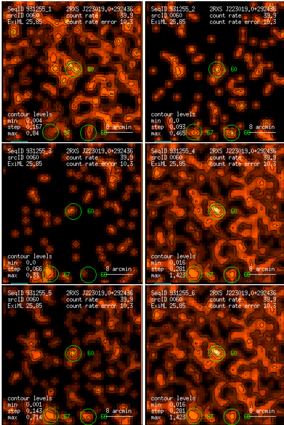
Figure 60: RASS 931255: detection 0060: band rate images, Gaussian filter: (1) PSPC channels 11 – 41, (2) 52 – 90, (3) 91 – 201, (4) 11 – 235, (5) 52 – 201, (6) 11 – 201. Broad band rates in counts/ks. Band rate contour levels in counts/ks/arcmin 2 .
