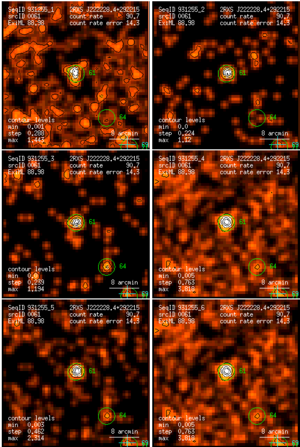
Figure 61: RASS 931255: detection 0061: band rate images, Gaussian filter: (1) PSPC channels 11 – 41, (2) 52 – 90, (3) 91 – 201, (4) 11 – 235, (5) 52 – 201, (6) 11 – 201. Broad band rates in counts/ks. Band rate contour levels in counts/ks/arcmin 2 .
