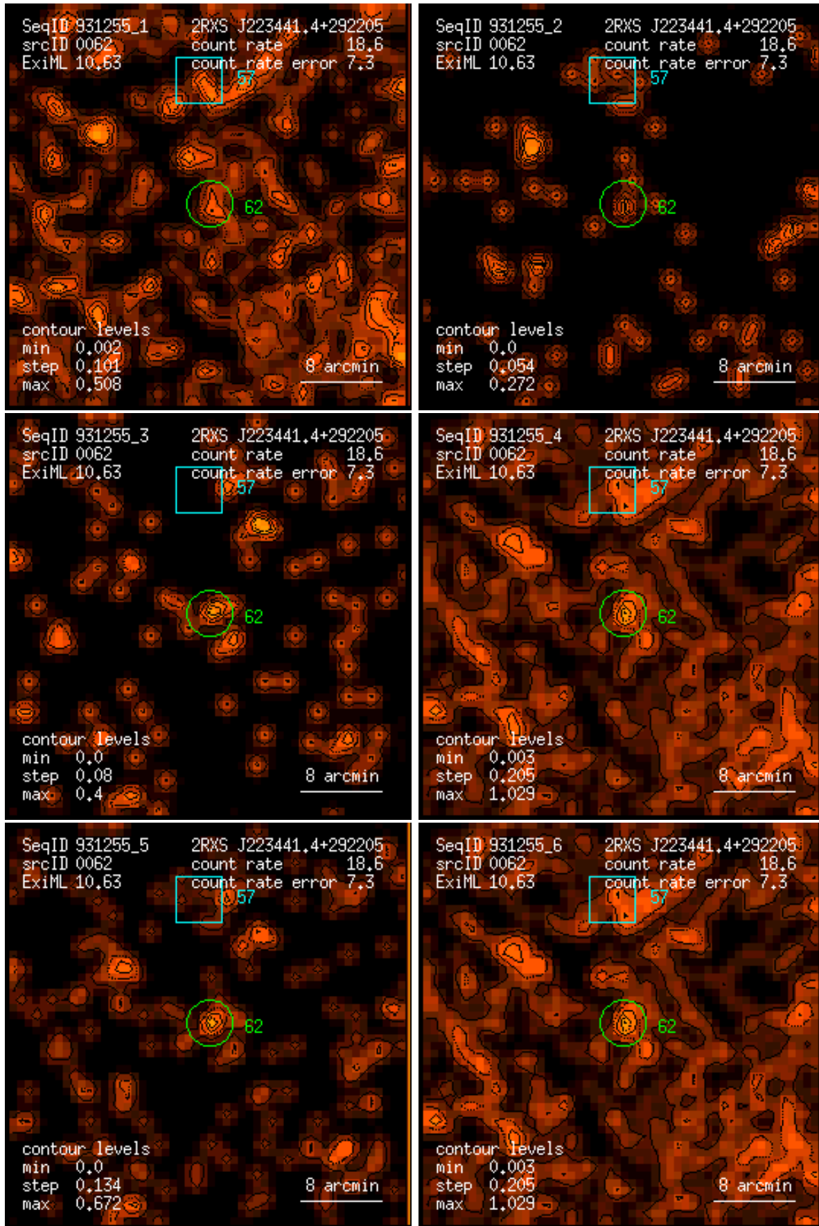
Figure 62: RASS 931255: detection 0062: band rate images, Gaussian filter: (1) PSPC channels 11 – 41, (2) 52 – 90, (3) 91 – 201, (4) 11 – 235, (5) 52 – 201, (6) 11 – 201. Broad band rates in counts/ks. Band rate contour levels in counts/ks/arcmin 2 .
