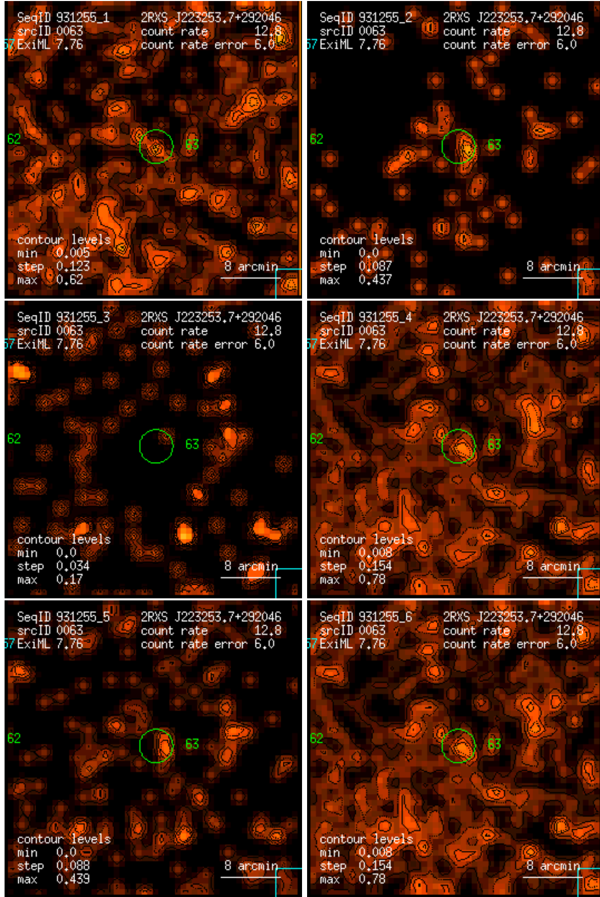
Figure 63: RASS 931255: detection 0063: band rate images, Gaussian filter: (1) PSPC channels 11 – 41, (2) 52 – 90, (3) 91 – 201, (4) 11 – 235, (5) 52 – 201, (6) 11 – 201. Broad band rates in counts/ks. Band rate contour levels in counts/ks/arcmin 2 .
