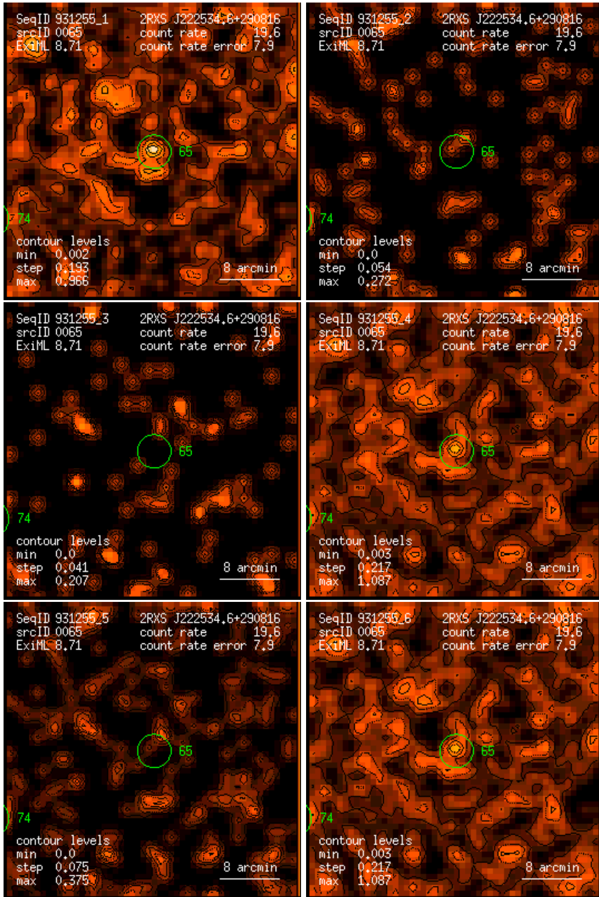
Figure 65: RASS 931255: detection 0065: band rate images, Gaussian filter: (1) PSPC channels 11 – 41, (2) 52 – 90, (3) 91 – 201, (4) 11 – 235, (5) 52 – 201, (6) 11 – 201. Broad band rates in counts/ks. Band rate contour levels in counts/ks/arcmin 2 .
