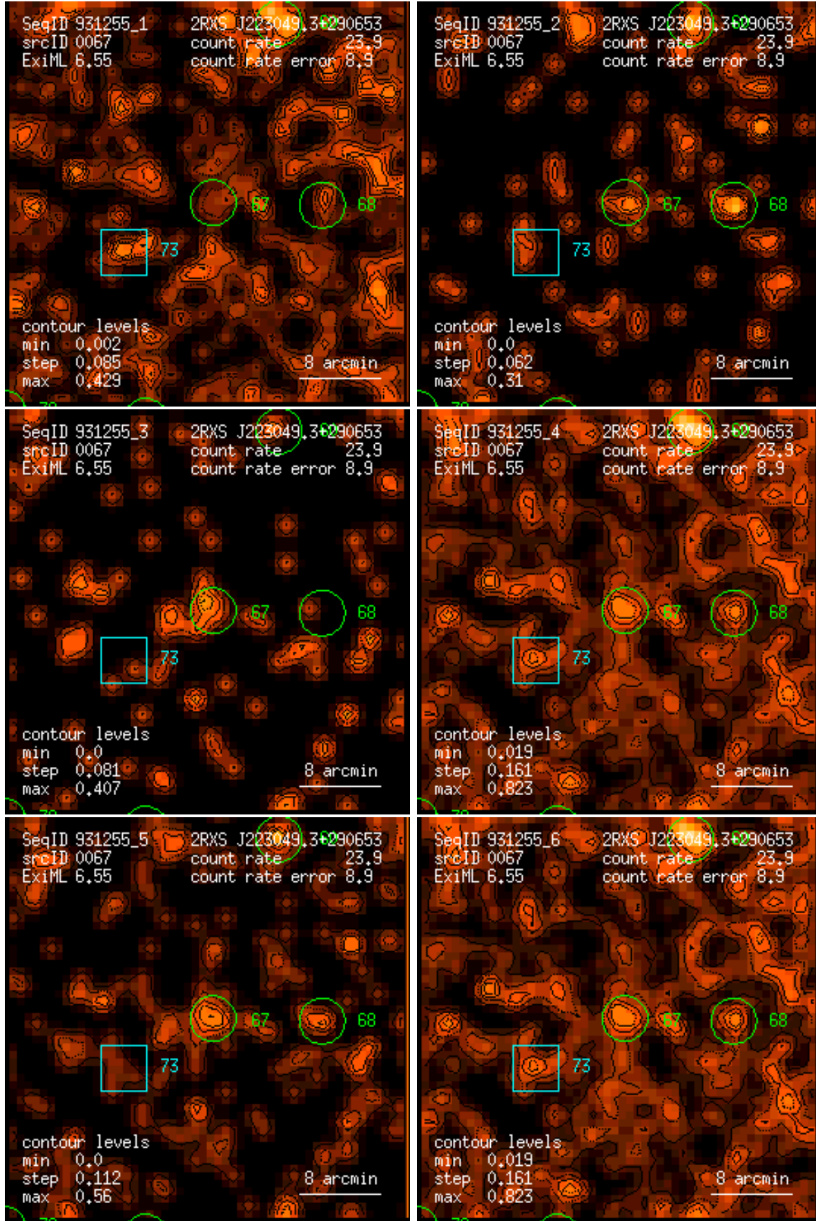
Figure 67: RASS 931255: detection 0067: band rate images, Gaussian filter: (1) PSPC channels 11 – 41, (2) 52 – 90, (3) 91 – 201, (4) 11 – 235, (5) 52 – 201, (6) 11 – 201. Broad band rates in counts/ks. Band rate contour levels in counts/ks/arcmin 2 .
