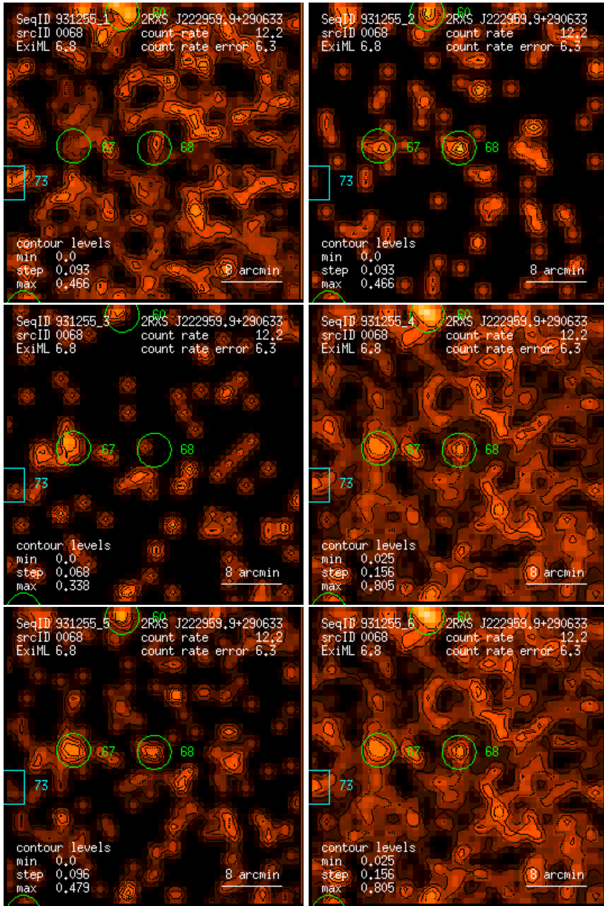
Figure 68: RASS 931255: detection 0068: band rate images, Gaussian filter: (1) PSPC channels 11 – 41, (2) 52 – 90, (3) 91 – 201, (4) 11 – 235, (5) 52 – 201, (6) 11 – 201. Broad band rates in counts/ks. Band rate contour levels in counts/ks/arcmin 2 .
