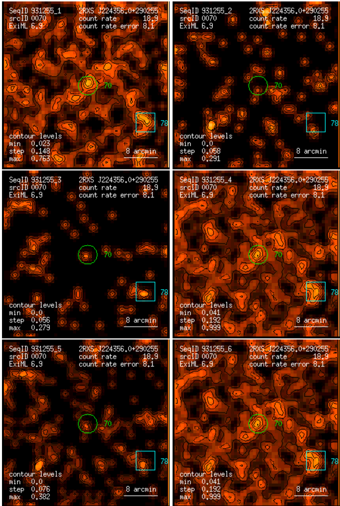
Figure 70: RASS 931255: detection 0070: band rate images, Gaussian filter: (1) PSPC channels 11 – 41, (2) 52 – 90, (3) 91 – 201, (4) 11 – 235, (5) 52 – 201, (6) 11 – 201. Broad band rates in counts/ks. Band rate contour levels in counts/ks/arcmin 2 .
