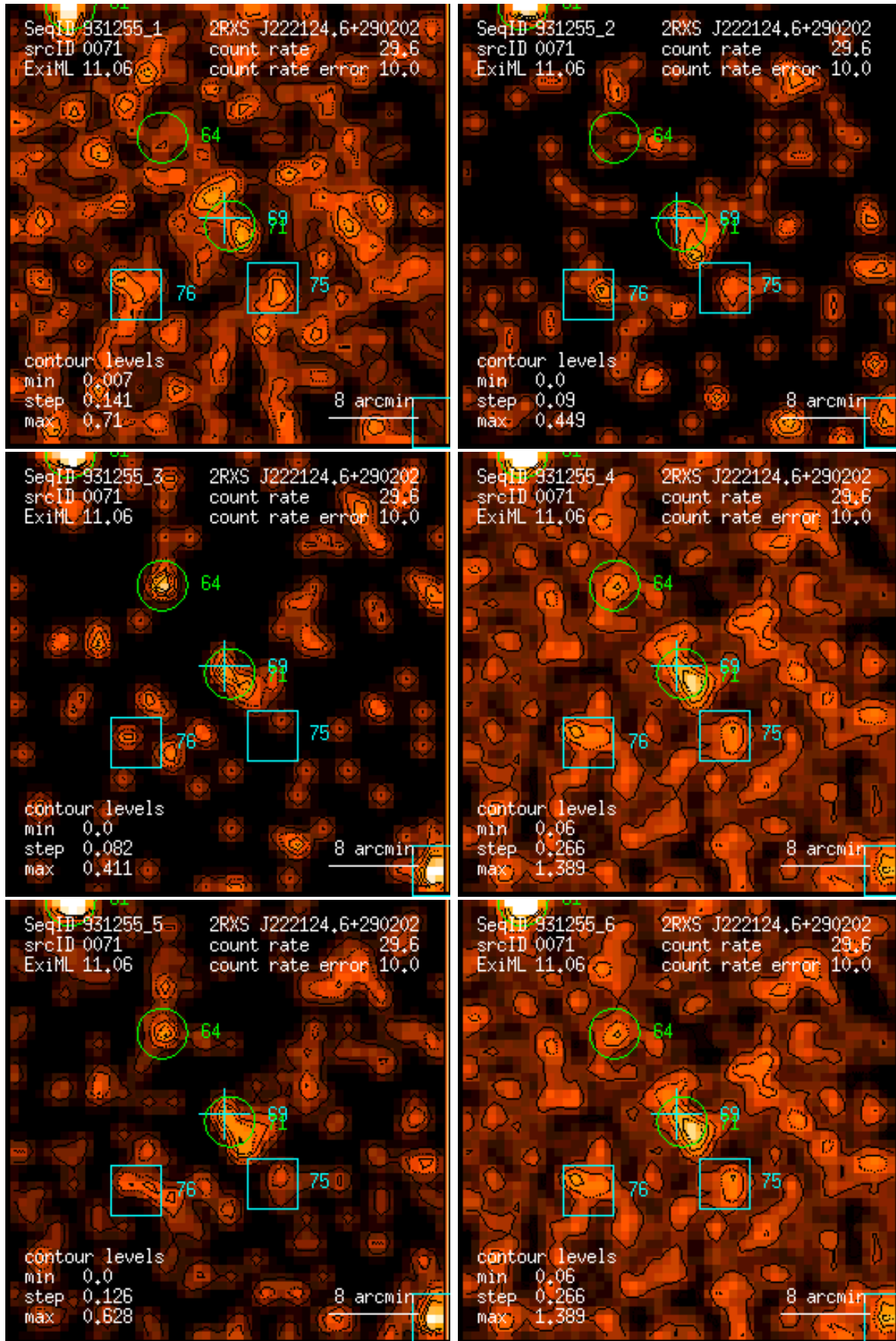
Figure 71: RASS 931255: detection 0071: band rate images, Gaussian filter: (1) PSPC channels 11 – 41, (2) 52 – 90, (3) 91 – 201, (4) 11 – 235, (5) 52 – 201, (6) 11 – 201. Broad band rates in counts/ks. Band rate contour levels in counts/ks/arcmin 2 .
