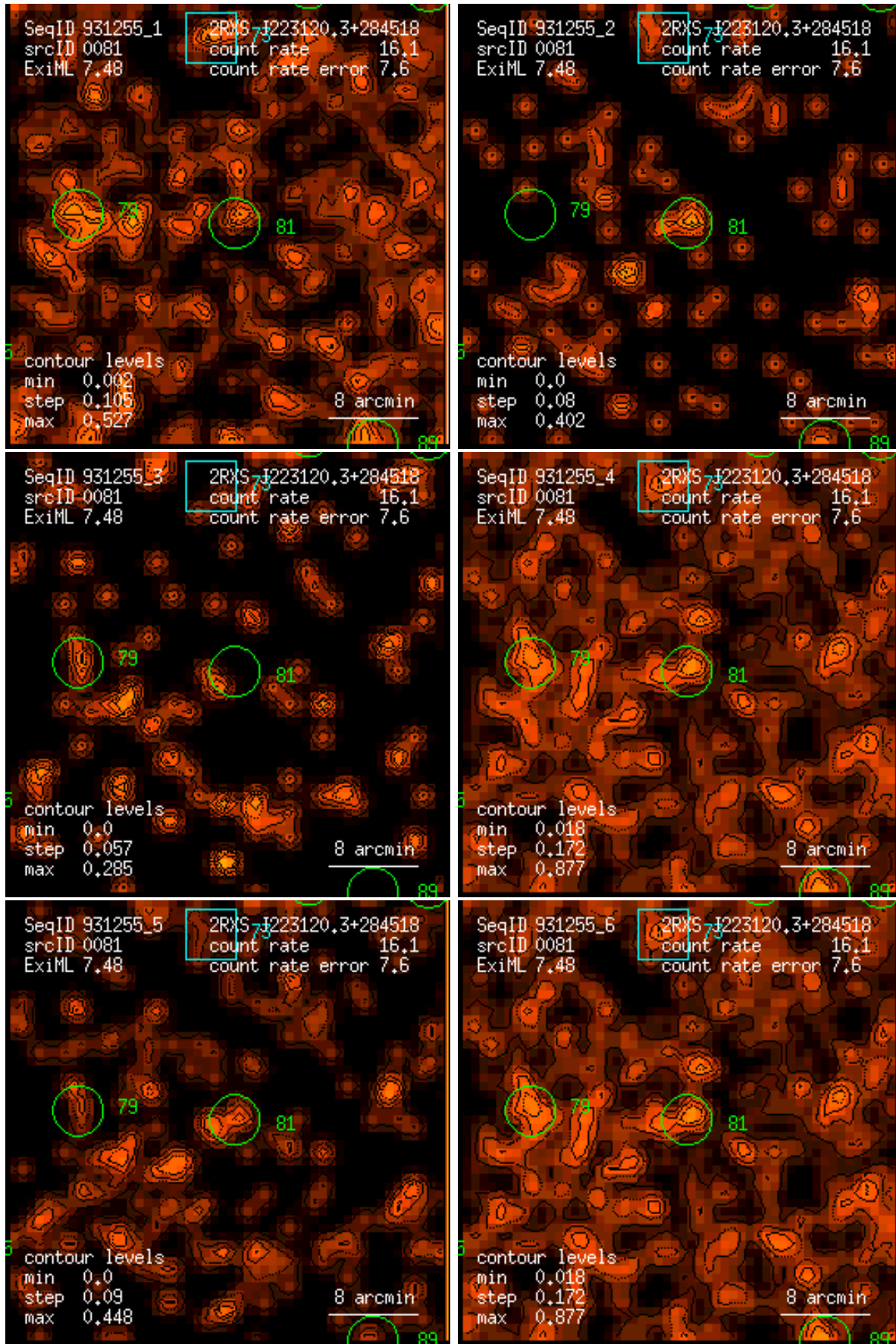
Figure 81: RASS 931255: detection 0081: band rate images, Gaussian filter: (1) PSPC channels 11 – 41, (2) 52 – 90, (3) 91 – 201, (4) 11 – 235, (5) 52 – 201, (6) 11 – 201. Broad band rates in counts/ks. Band rate contour levels in counts/ks/arcmin 2 .
