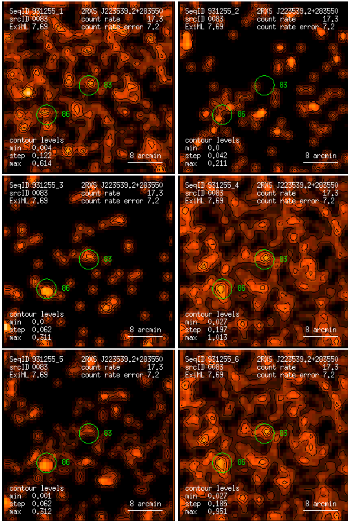
Figure 83: RASS 931255: detection 0083: band rate images, Gaussian filter: (1) PSPC channels 11 – 41, (2) 52 – 90, (3) 91 – 201, (4) 11 – 235, (5) 52 – 201, (6) 11 – 201. Broad band rates in counts/ks. Band rate contour levels in counts/ks/arcmin 2 .
