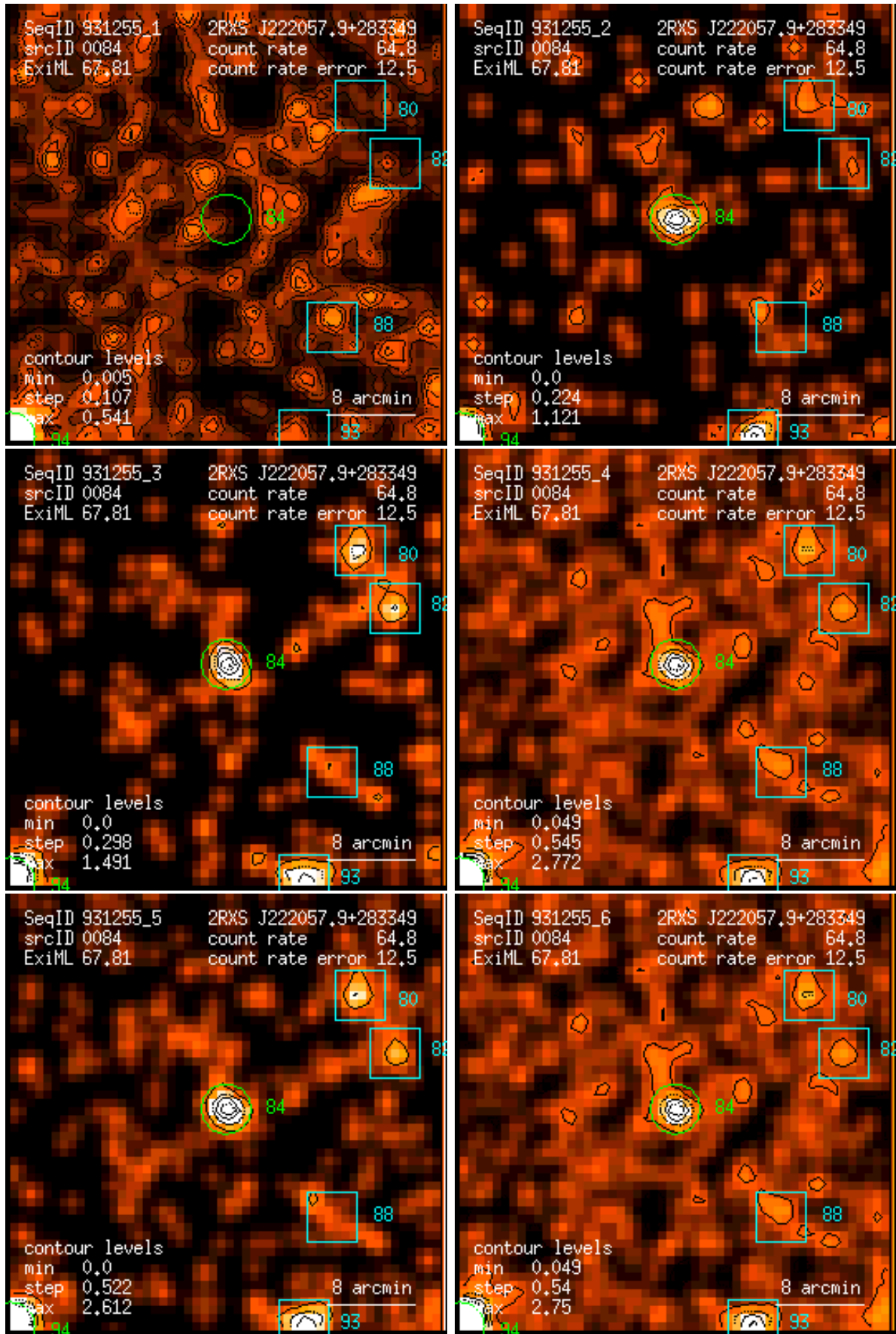
Figure 84: RASS 931255: detection 0084: band rate images, Gaussian filter: (1) PSPC channels 11 – 41, (2) 52 – 90, (3) 91 – 201, (4) 11 – 235, (5) 52 – 201, (6) 11 – 201. Broad band rates in counts/ks. Band rate contour levels in counts/ks/arcmin 2 .
