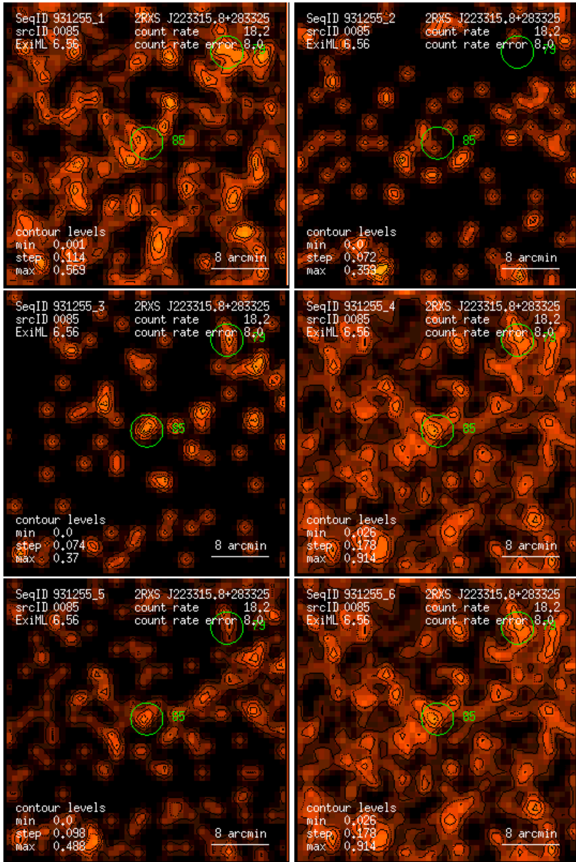
Figure 85: RASS 931255: detection 0085: band rate images, Gaussian filter: (1) PSPC channels 11 – 41, (2) 52 – 90, (3) 91 – 201, (4) 11 – 235, (5) 52 – 201, (6) 11 – 201. Broad band rates in counts/ks. Band rate contour levels in counts/ks/arcmin 2 .
