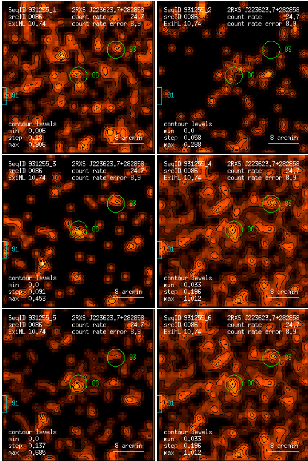
Figure 86: RASS 931255: detection 0086: band rate images, Gaussian filter: (1) PSPC channels 11 – 41, (2) 52 – 90, (3) 91 – 201, (4) 11 – 235, (5) 52 – 201, (6) 11 – 201. Broad band rates in counts/ks. Band rate contour levels in counts/ks/arcmin 2 .
