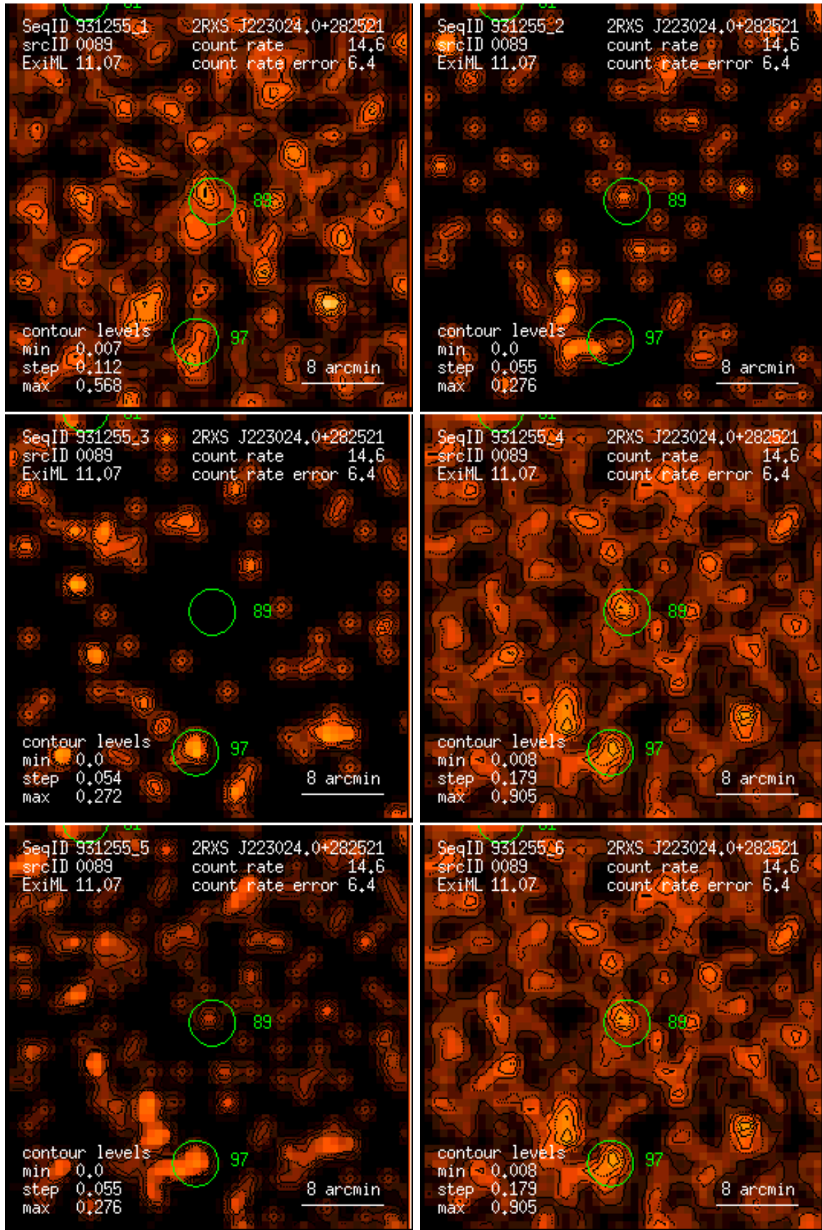
Figure 89: RASS 931255: detection 0089: band rate images, Gaussian filter: (1) PSPC channels 11 – 41, (2) 52 – 90, (3) 91 – 201, (4) 11 – 235, (5) 52 – 201, (6) 11 – 201. Broad band rates in counts/ks. Band rate contour levels in counts/ks/arcmin 2 .
