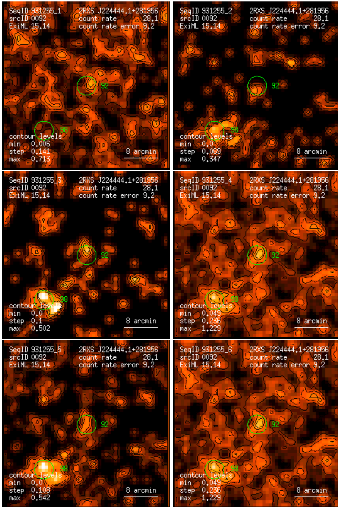
Figure 92: RASS 931255: detection 0092: band rate images, Gaussian filter: (1) PSPC channels 11 – 41, (2) 52 – 90, (3) 91 – 201, (4) 11 – 235, (5) 52 – 201, (6) 11 – 201. Broad band rates in counts/ks. Band rate contour levels in counts/ks/arcmin 2 .
