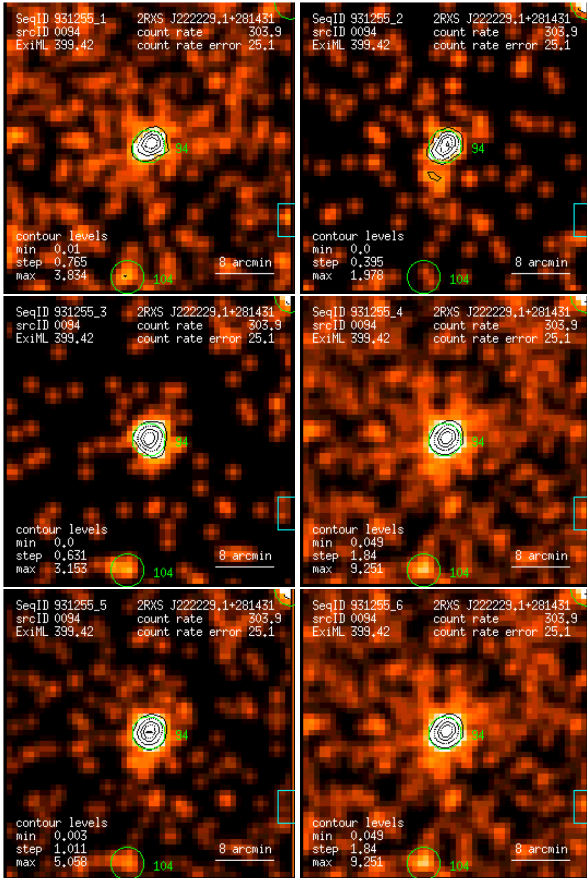
Figure 94: RASS 931255: detection 0094: band rate images, Gaussian filter: (1) PSPC channels 11 – 41, (2) 52 – 90, (3) 91 – 201, (4) 11 – 235, (5) 52 – 201, (6) 11 – 201. Broad band rates in counts/ks. Band rate contour levels in counts/ks/arcmin 2 .
