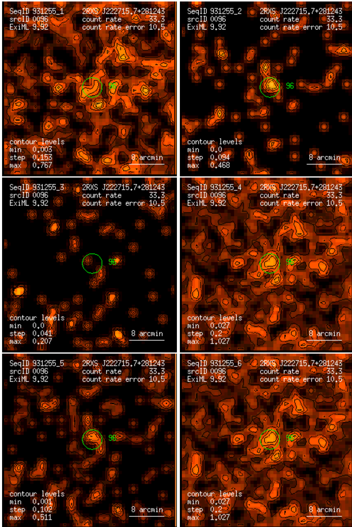
Figure 96: RASS 931255: detection 0096: band rate images, Gaussian filter: (1) PSPC channels 11 – 41, (2) 52 – 90, (3) 91 – 201, (4) 11 – 235, (5) 52 – 201, (6) 11 – 201. Broad band rates in counts/ks. Band rate contour levels in counts/ks/arcmin 2 .
