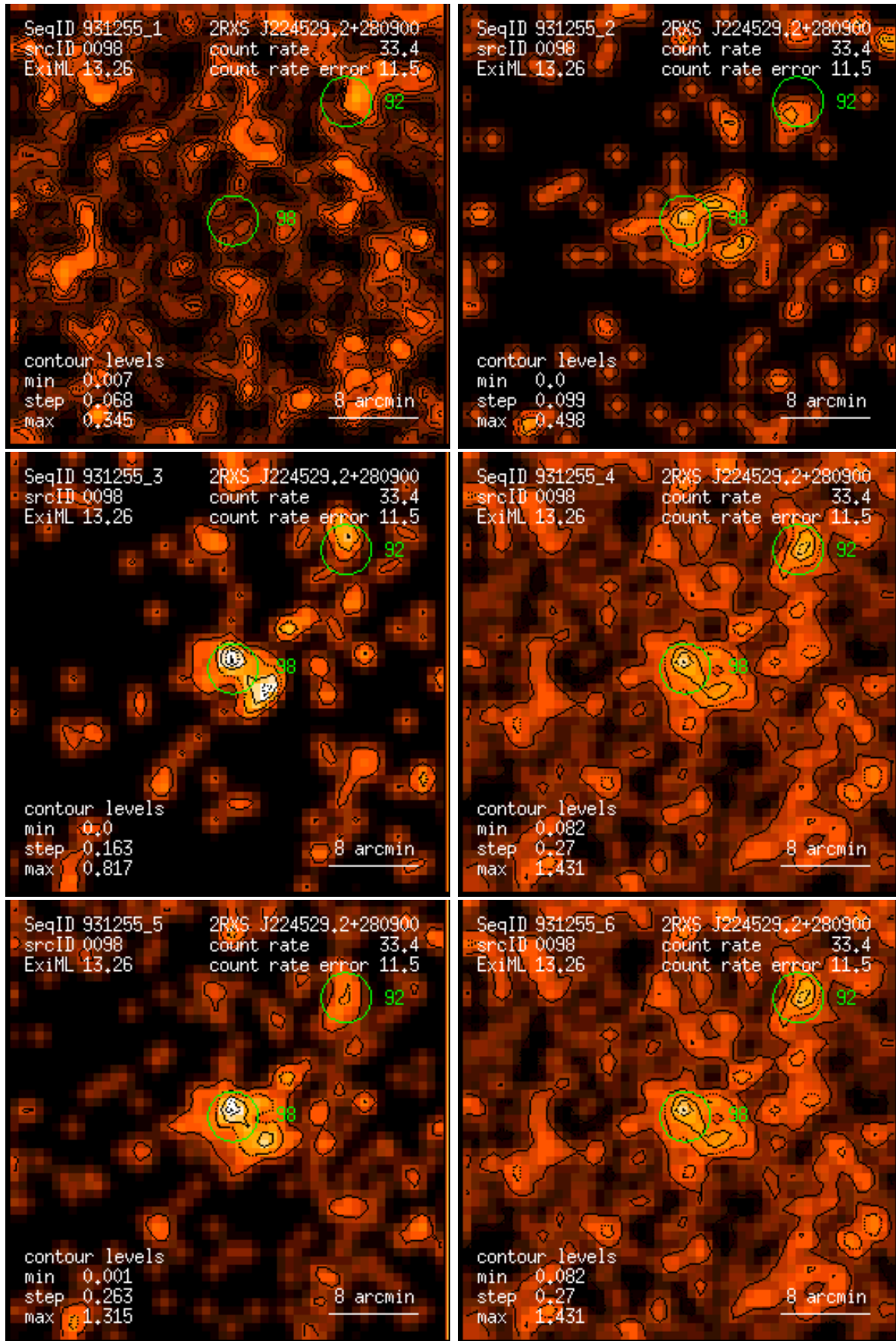
Figure 98: RASS 931255: detection 0098: band rate images, Gaussian filter: (1) PSPC channels 11 – 41, (2) 52 – 90, (3) 91 – 201, (4) 11 – 235, (5) 52 – 201, (6) 11 – 201. Broad band rates in counts/ks. Band rate contour levels in counts/ks/arcmin 2 .
