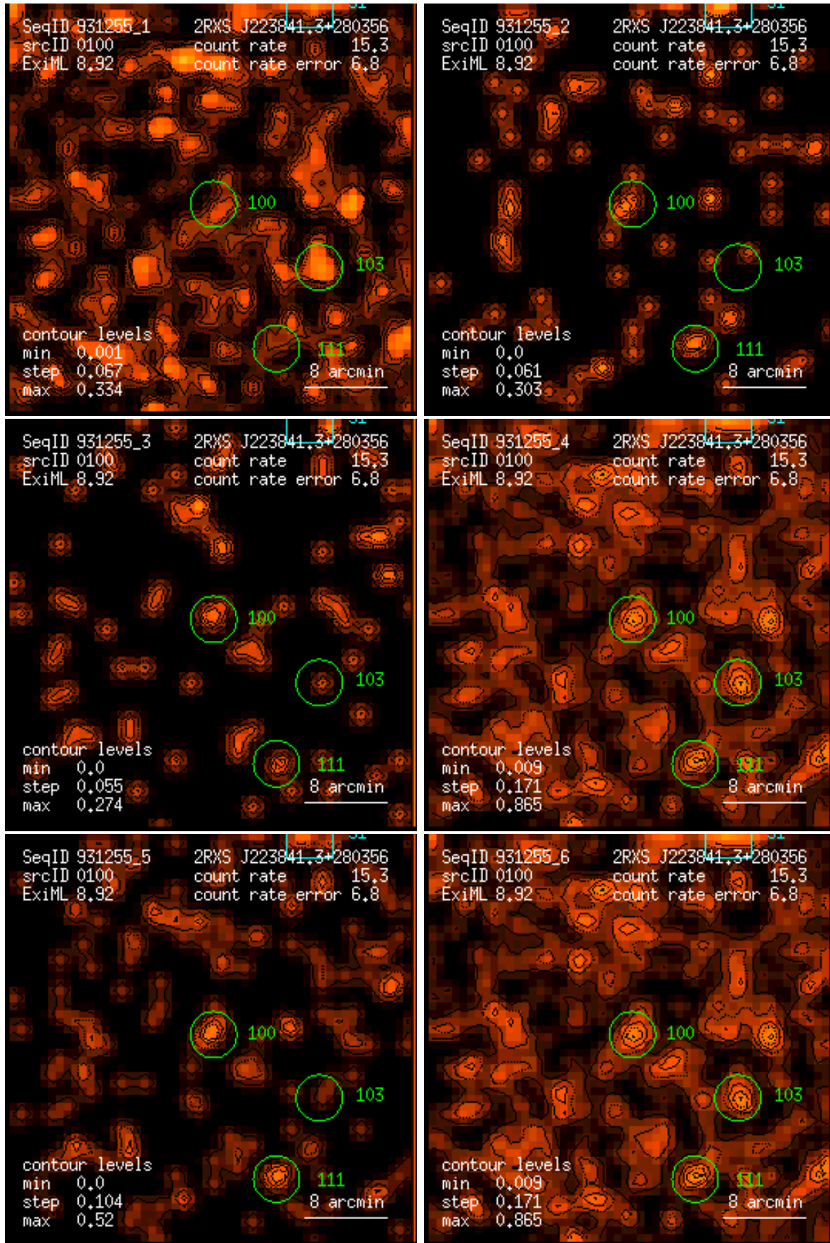
Figure 100: RASS 931255: detection 0100: band rate images, Gaussian filter: (1) PSPC channels 11 – 41, (2) 52 – 90, (3) 91 – 201, (4) 11 – 235, (5) 52 – 201, (6) 11 – 201. Broad band rates in counts/ks. Band rate contour levels in counts/ks/arcmin 2 .
