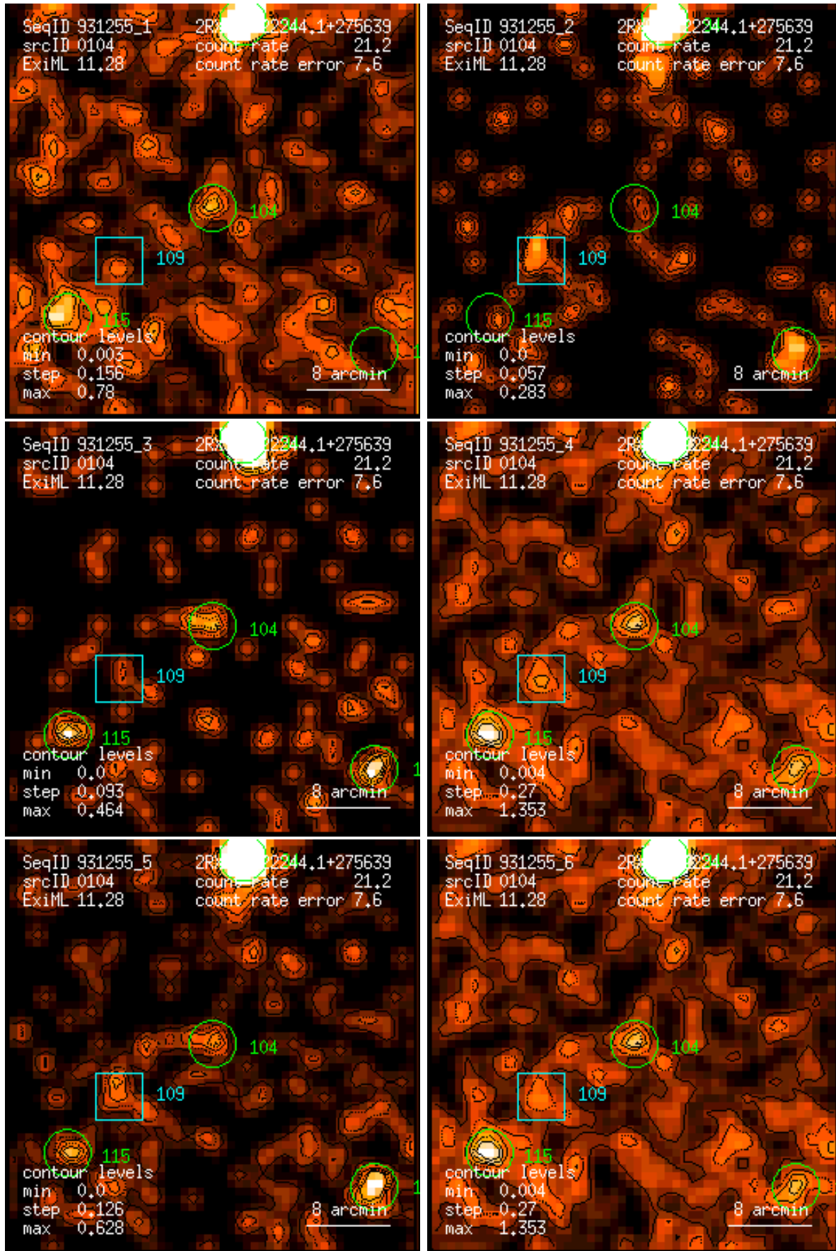
Figure 104: RASS 931255: detection 0104: band rate images, Gaussian filter: (1) PSPC channels 11 – 41, (2) 52 – 90, (3) 91 – 201, (4) 11 – 235, (5) 52 – 201, (6) 11 – 201. Broad band rates in counts/ks. Band rate contour levels in counts/ks/arcmin 2 .
