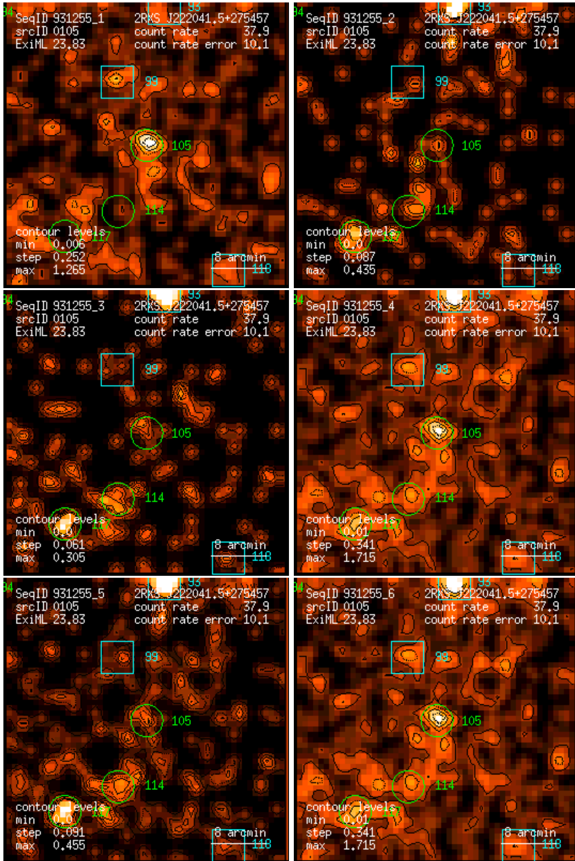
Figure 105: RASS 931255: detection 0105: band rate images, Gaussian filter: (1) PSPC channels 11 – 41, (2) 52 – 90, (3) 91 – 201, (4) 11 – 235, (5) 52 – 201, (6) 11 – 201. Broad band rates in counts/ks. Band rate contour levels in counts/ks/arcmin 2 .
