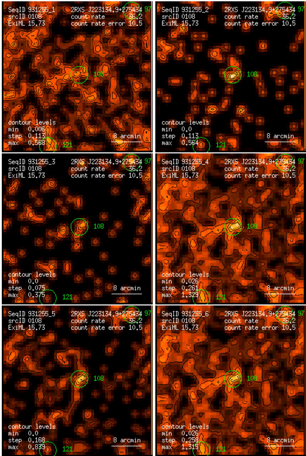
Figure 108: RASS 931255: detection 0108: band rate images, Gaussian filter: (1) PSPC channels 11 – 41, (2) 52 – 90, (3) 91 – 201, (4) 11 – 235, (5) 52 – 201, (6) 11 – 201. Broad band rates in counts/ks. Band rate contour levels in counts/ks/arcmin 2 .
