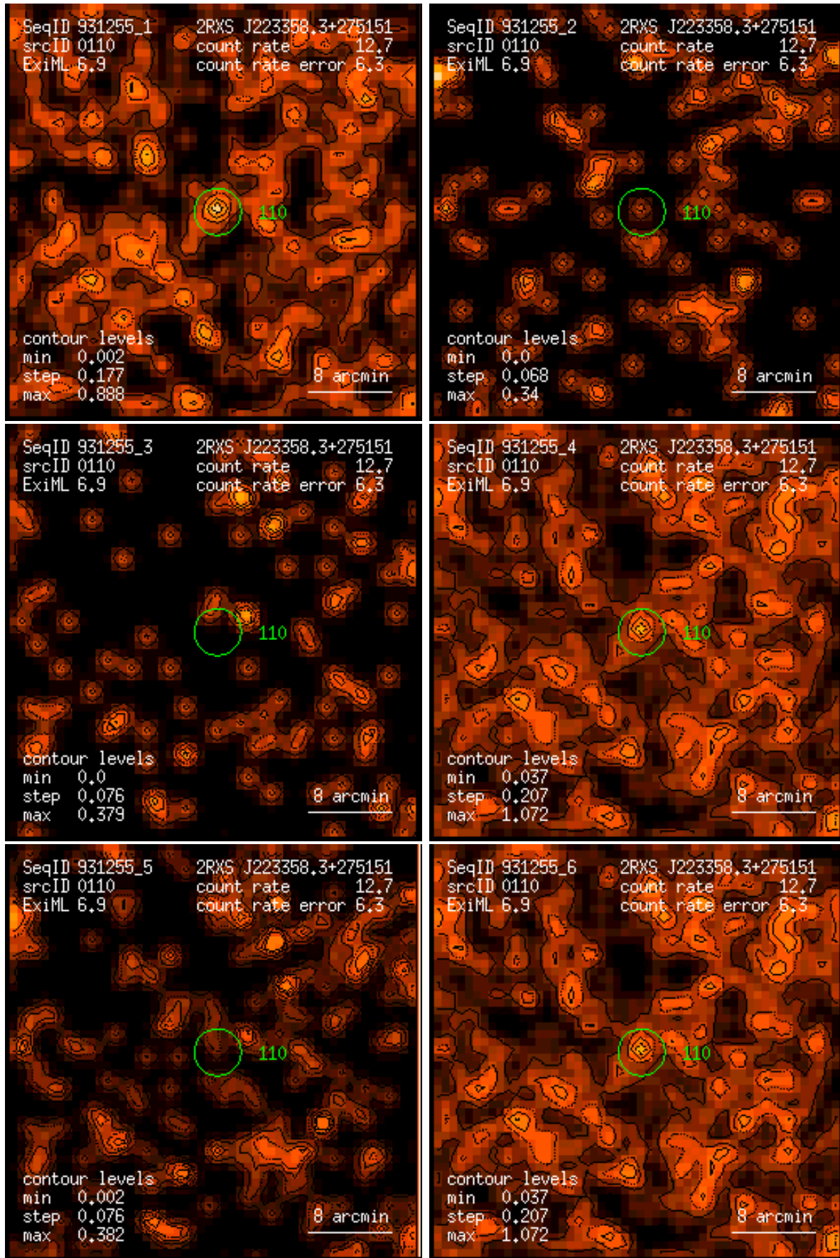
Figure 110: RASS 931255: detection 0110: band rate images, Gaussian filter: (1) PSPC channels 11 – 41, (2) 52 – 90, (3) 91 – 201, (4) 11 – 235, (5) 52 – 201, (6) 11 – 201. Broad band rates in counts/ks. Band rate contour levels in counts/ks/arcmin 2 .
