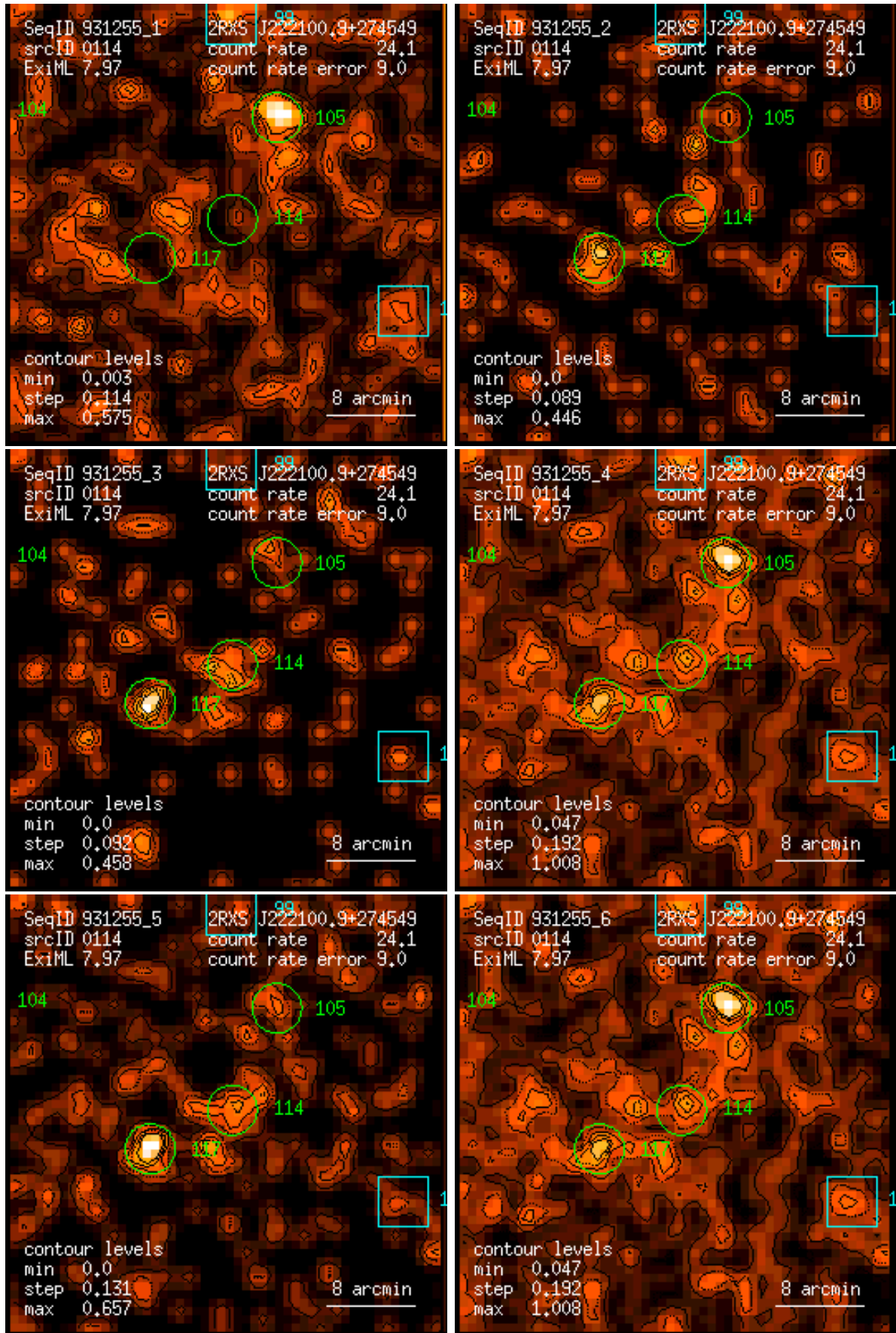
Figure 114: RASS 931255: detection 0114: band rate images, Gaussian filter: (1) PSPC channels 11 – 41, (2) 52 – 90, (3) 91 – 201, (4) 11 – 235, (5) 52 – 201, (6) 11 – 201. Broad band rates in counts/ks. Band rate contour levels in counts/ks/arcmin 2 .
