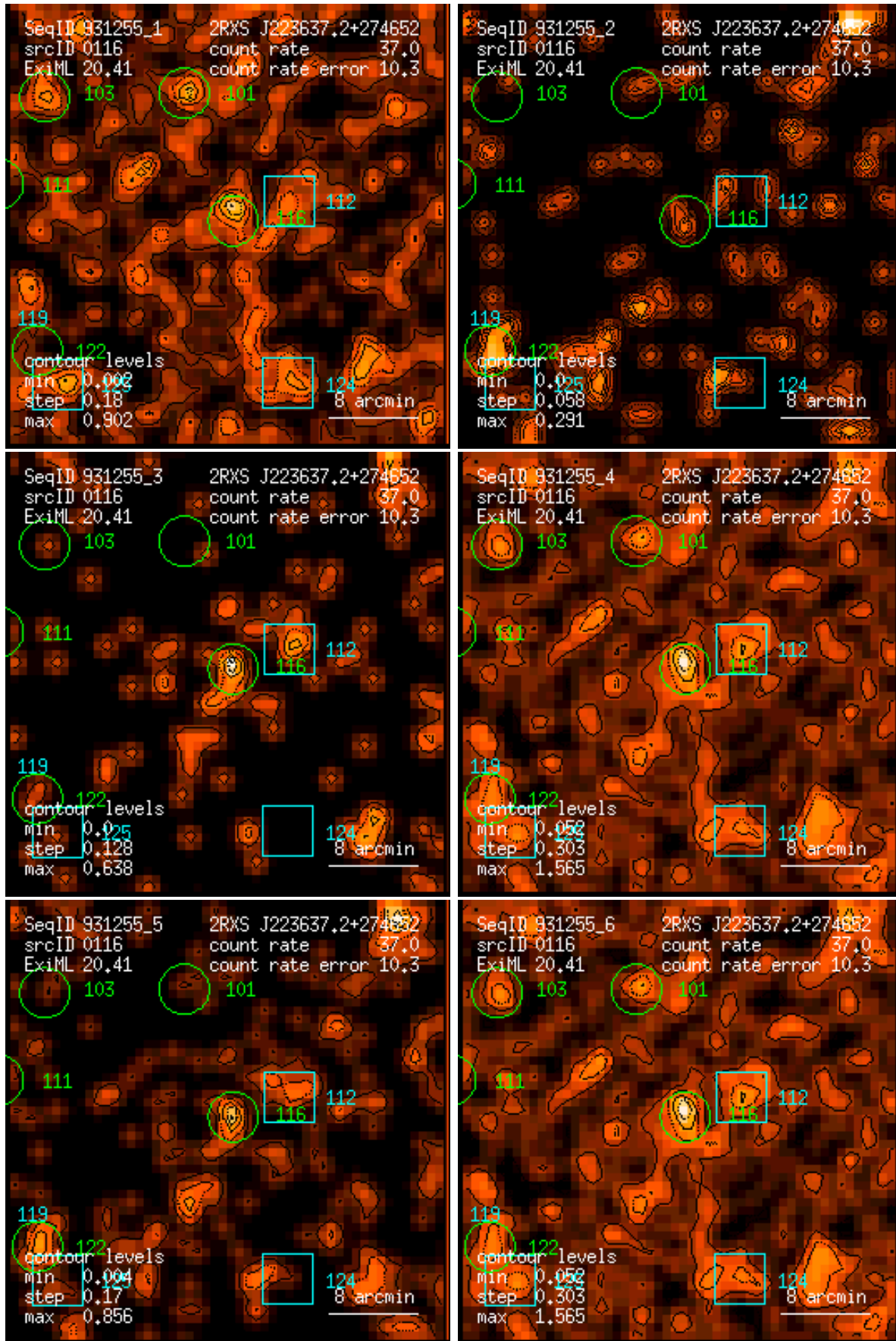
Figure 116: RASS 931255: detection 0116: band rate images, Gaussian filter: (1) PSPC channels 11 – 41, (2) 52 – 90, (3) 91 – 201, (4) 11 – 235, (5) 52 – 201, (6) 11 – 201. Broad band rates in counts/ks. Band rate contour levels in counts/ks/arcmin 2 .
