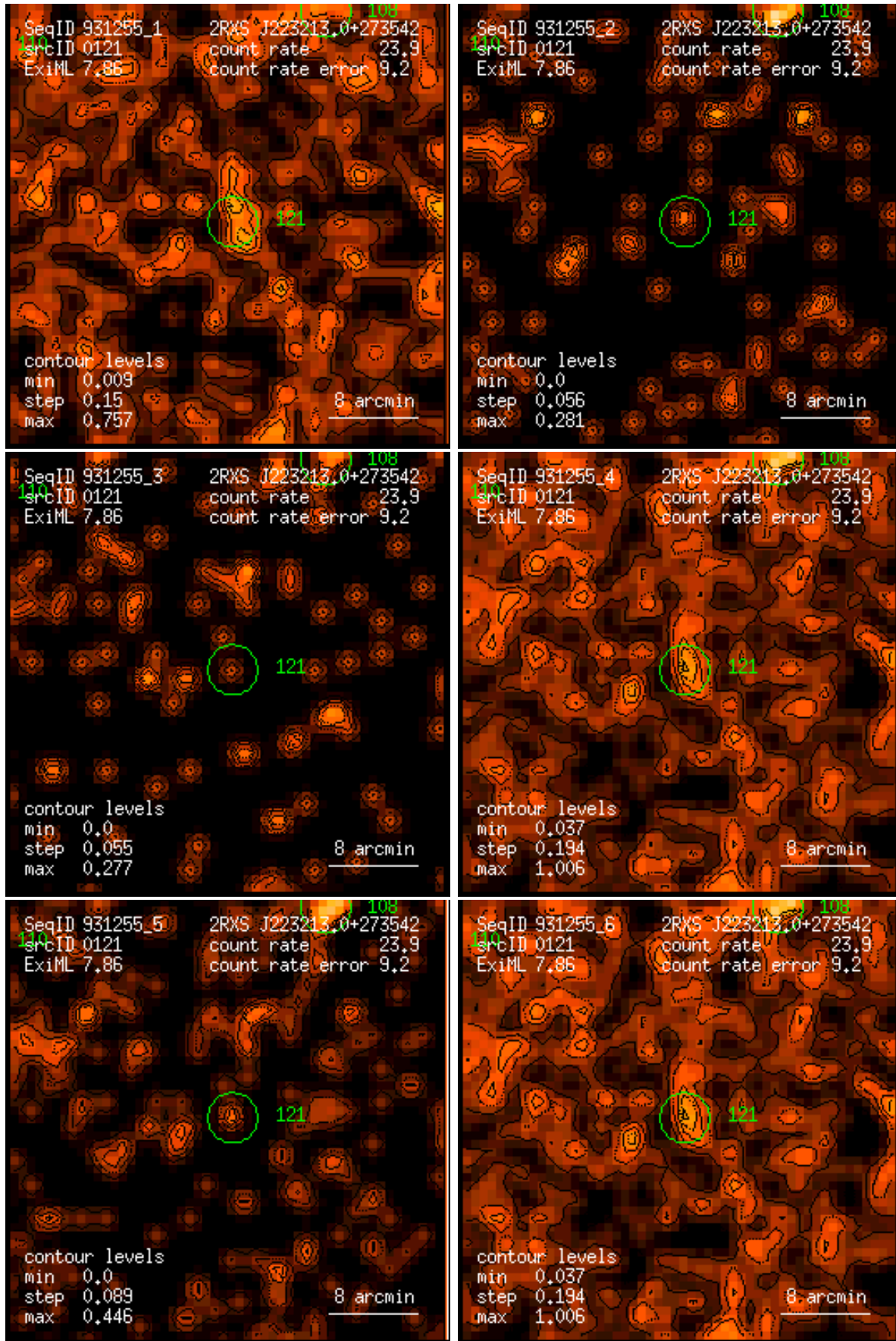
Figure 121: RASS 931255: detection 0121: band rate images, Gaussian filter: (1) PSPC channels 11 – 41, (2) 52 – 90, (3) 91 – 201, (4) 11 – 235, (5) 52 – 201, (6) 11 – 201. Broad band rates in counts/ks. Band rate contour levels in counts/ks/arcmin 2 .
