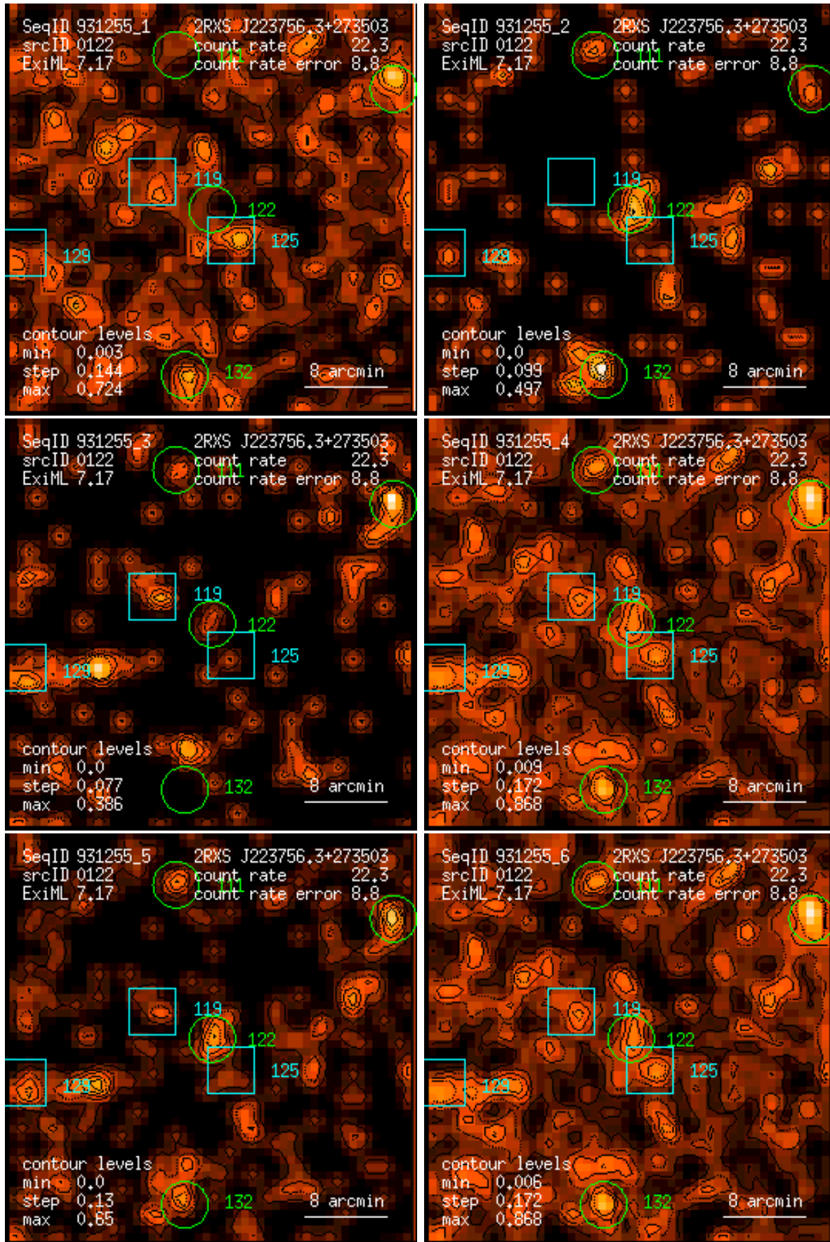
Figure 122: RASS 931255: detection 0122: band rate images, Gaussian filter: (1) PSPC channels 11 – 41, (2) 52 – 90, (3) 91 – 201, (4) 11 – 235, (5) 52 – 201, (6) 11 – 201. Broad band rates in counts/ks. Band rate contour levels in counts/ks/arcmin 2 .
