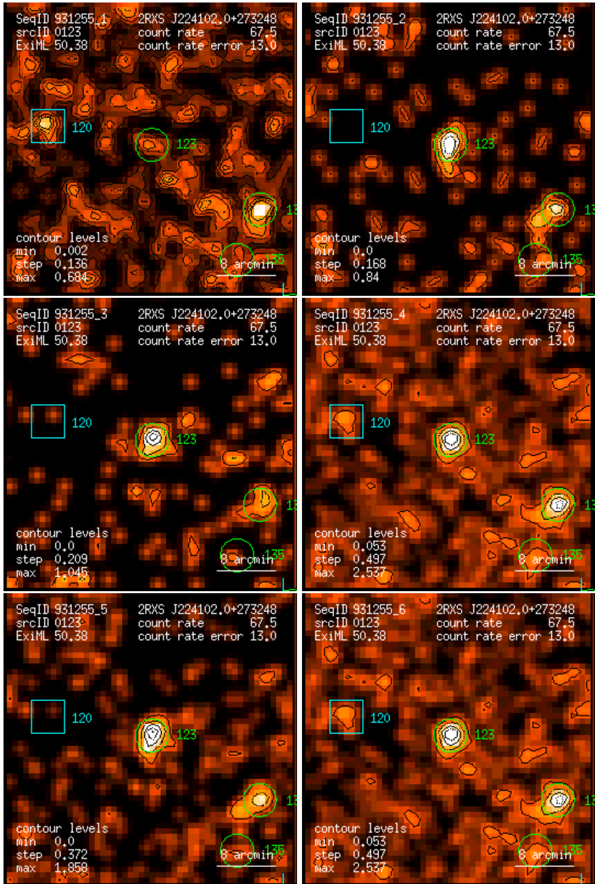
Figure 123: RASS 931255: detection 0123: band rate images, Gaussian filter: (1) PSPC channels 11 – 41, (2) 52 – 90, (3) 91 – 201, (4) 11 – 235, (5) 52 – 201, (6) 11 – 201. Broad band rates in counts/ks. Band rate contour levels in counts/ks/arcmin 2 .
