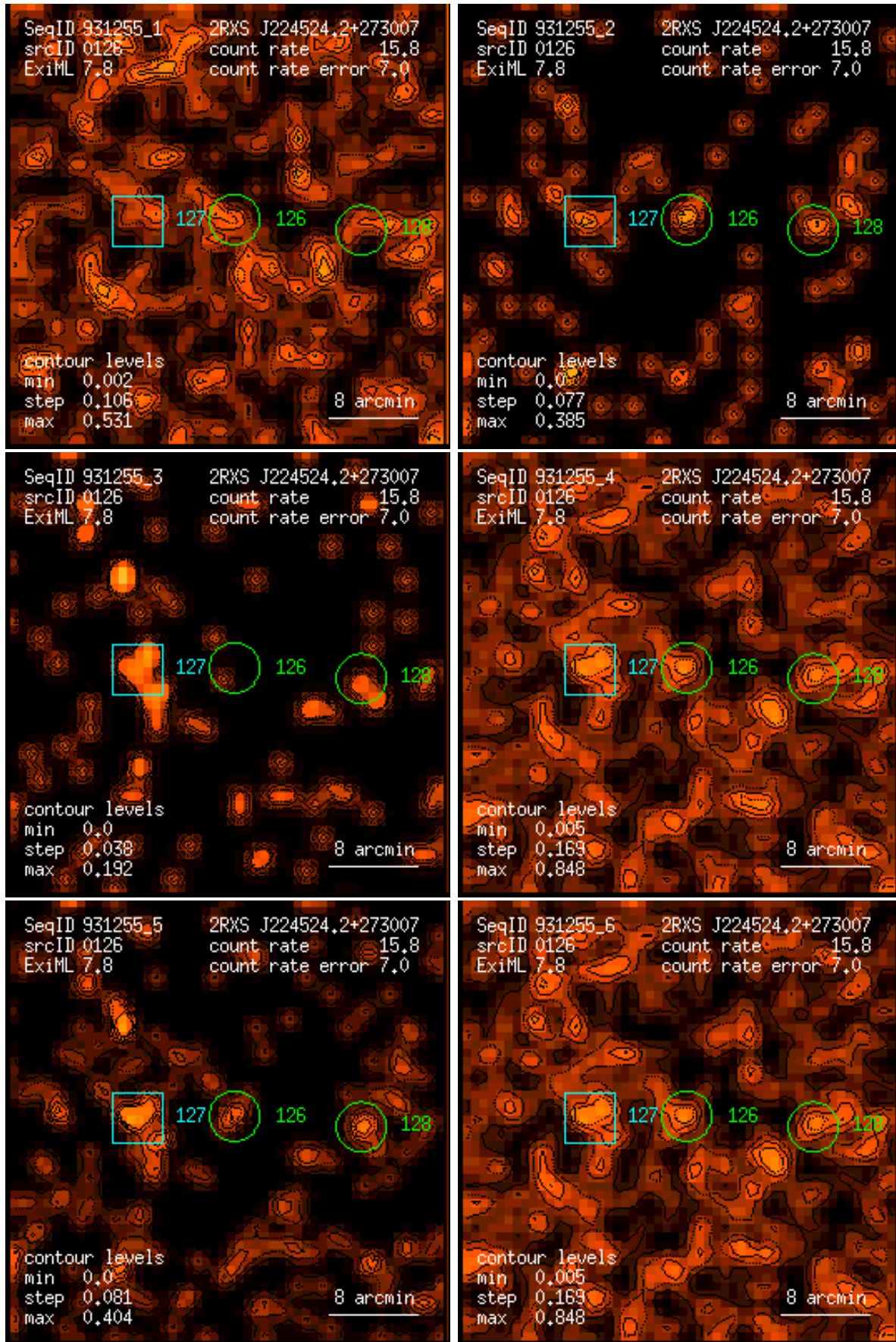
Figure 126: RASS 931255: detection 0126: band rate images, Gaussian filter: (1) PSPC channels 11 – 41, (2) 52 – 90, (3) 91 – 201, (4) 11 – 235, (5) 52 – 201, (6) 11 – 201. Broad band rates in counts/ks. Band rate contour levels in counts/ks/arcmin 2 .
