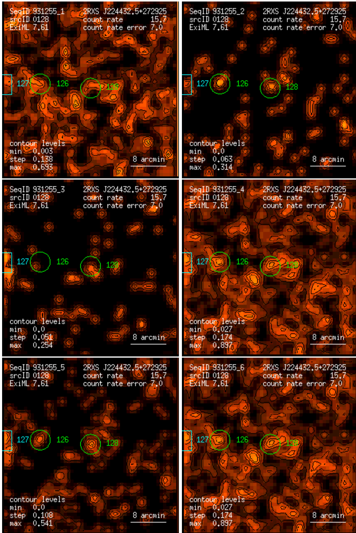
Figure 128: RASS 931255: detection 0128: band rate images, Gaussian filter: (1) PSPC channels 11 – 41, (2) 52 – 90, (3) 91 – 201, (4) 11 – 235, (5) 52 – 201, (6) 11 – 201. Broad band rates in counts/ks. Band rate contour levels in counts/ks/arcmin 2 .
