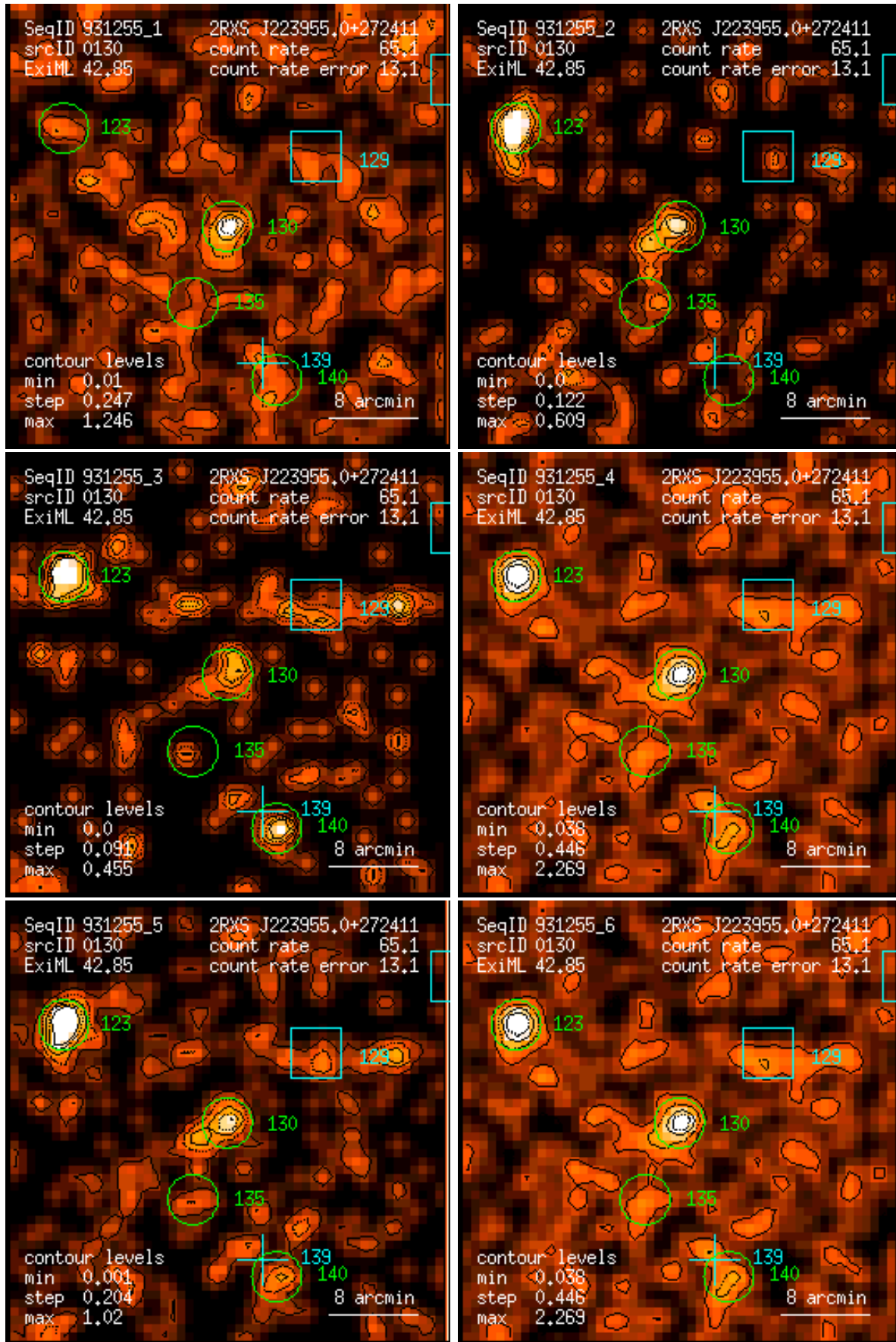
Figure 130: RASS 931255: detection 0130: band rate images, Gaussian filter: (1) PSPC channels 11 – 41, (2) 52 – 90, (3) 91 – 201, (4) 11 – 235, (5) 52 – 201, (6) 11 – 201. Broad band rates in counts/ks. Band rate contour levels in counts/ks/arcmin 2 .
