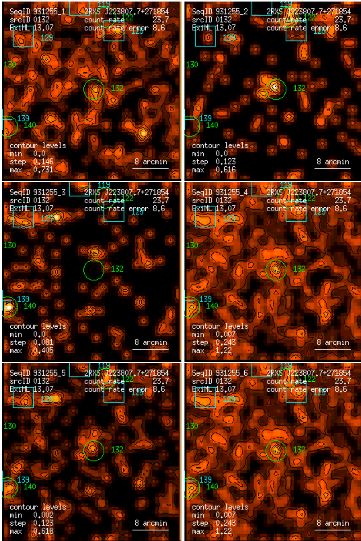
Figure 132: RASS 931255: detection 0132: band rate images, Gaussian filter: (1) PSPC channels 11 – 41, (2) 52 – 90, (3) 91 – 201, (4) 11 – 235, (5) 52 – 201, (6) 11 – 201. Broad band rates in counts/ks. Band rate contour levels in counts/ks/arcmin 2 .
