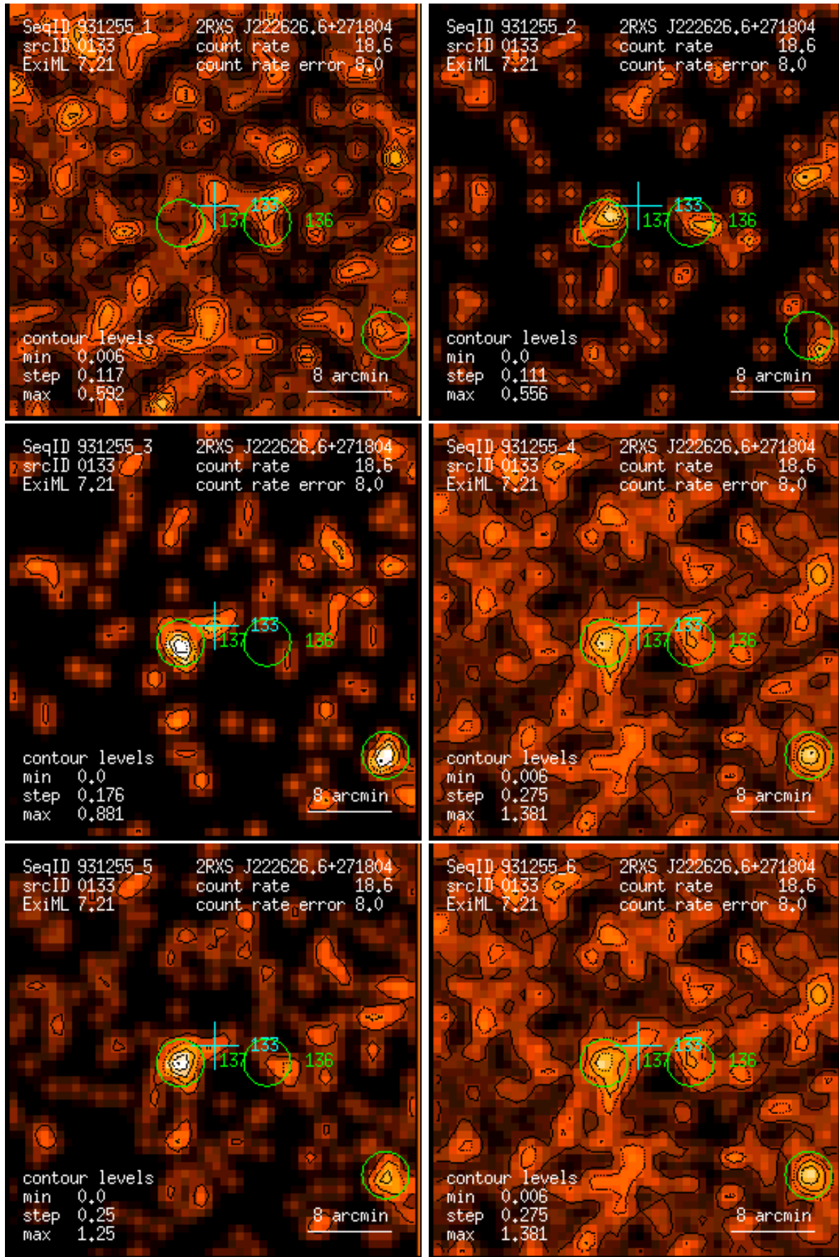
Figure 133: RASS 931255: detection 0133: band rate images, Gaussian filter: (1) PSPC channels 11 – 41, (2) 52 – 90, (3) 91 – 201, (4) 11 – 235, (5) 52 – 201, (6) 11 – 201. Broad band rates in counts/ks. Band rate contour levels in counts/ks/arcmin 2 .
