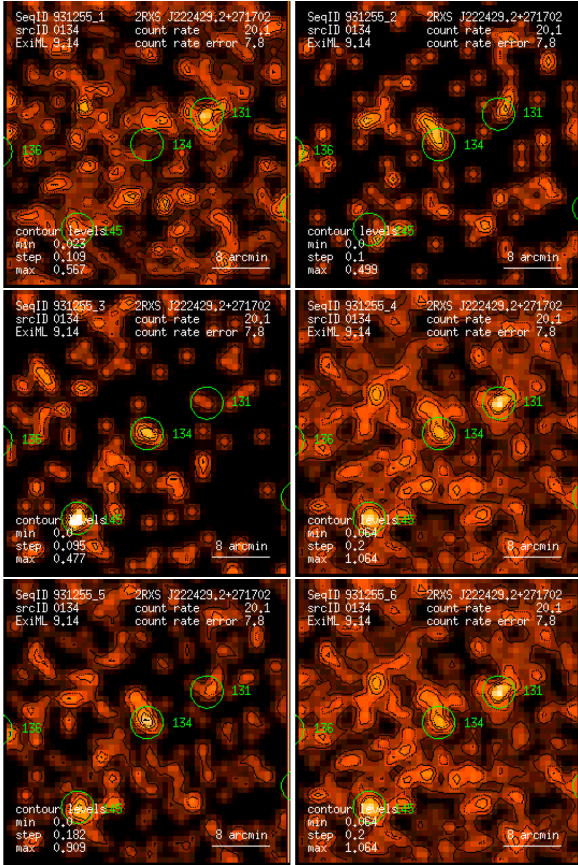
Figure 134: RASS 931255: detection 0134: band rate images, Gaussian filter: (1) PSPC channels 11 – 41, (2) 52 – 90, (3) 91 – 201, (4) 11 – 235, (5) 52 – 201, (6) 11 – 201. Broad band rates in counts/ks. Band rate contour levels in counts/ks/arcmin 2 .
