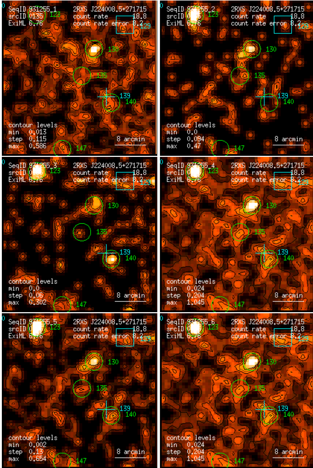
Figure 135: RASS 931255: detection 0135: band rate images, Gaussian filter: (1) PSPC channels 11 – 41, (2) 52 – 90, (3) 91 – 201, (4) 11 – 235, (5) 52 – 201, (6) 11 – 201. Broad band rates in counts/ks. Band rate contour levels in counts/ks/arcmin 2 .
