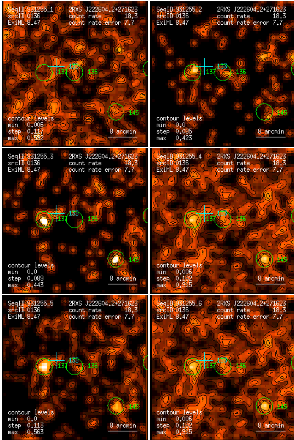
Figure 136: RASS 931255: detection 0136: band rate images, Gaussian filter: (1) PSPC channels 11 – 41, (2) 52 – 90, (3) 91 – 201, (4) 11 – 235, (5) 52 – 201, (6) 11 – 201. Broad band rates in counts/ks. Band rate contour levels in counts/ks/arcmin 2 .
