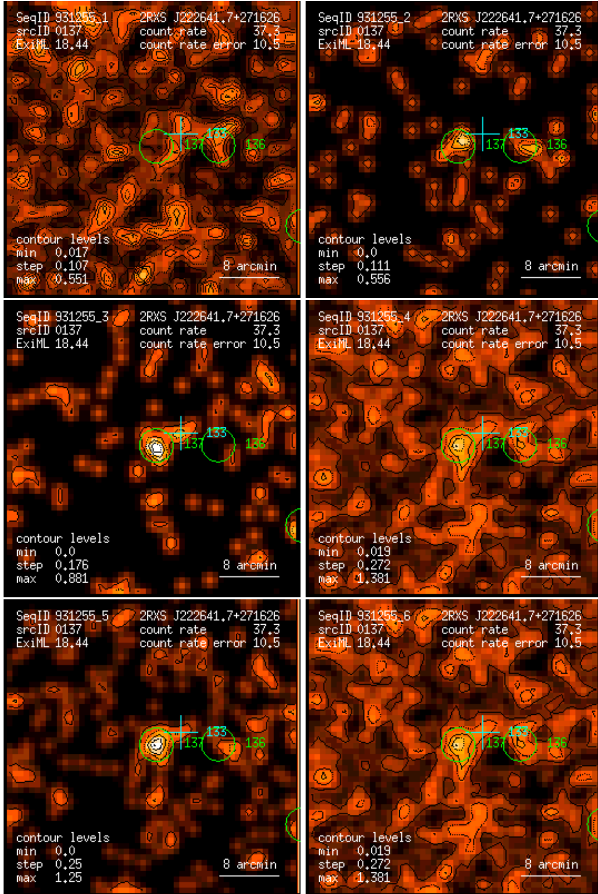
Figure 137: RASS 931255: detection 0137: band rate images, Gaussian filter: (1) PSPC channels 11 – 41, (2) 52 – 90, (3) 91 – 201, (4) 11 – 235, (5) 52 – 201, (6) 11 – 201. Broad band rates in counts/ks. Band rate contour levels in counts/ks/arcmin 2 .
