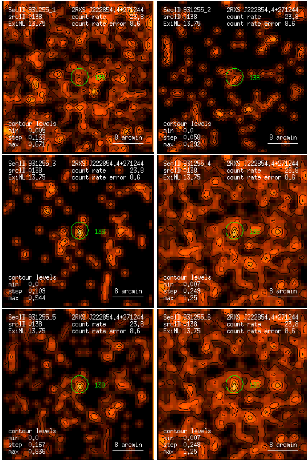
Figure 138: RASS 931255: detection 0138: band rate images, Gaussian filter: (1) PSPC channels 11 – 41, (2) 52 – 90, (3) 91 – 201, (4) 11 – 235, (5) 52 – 201, (6) 11 – 201. Broad band rates in counts/ks. Band rate contour levels in counts/ks/arcmin 2 .
