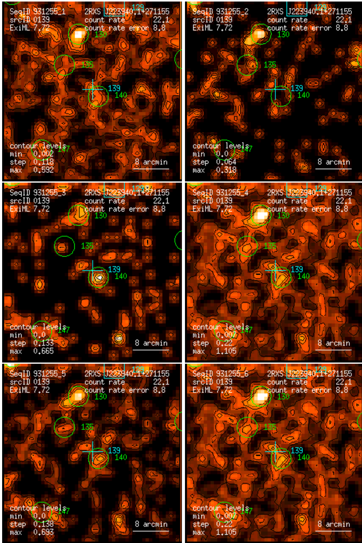
Figure 139: RASS 931255: detection 0139: band rate images, Gaussian filter: (1) PSPC channels 11 – 41, (2) 52 – 90, (3) 91 – 201, (4) 11 – 235, (5) 52 – 201, (6) 11 – 201. Broad band rates in counts/ks. Band rate contour levels in counts/ks/arcmin 2 .
