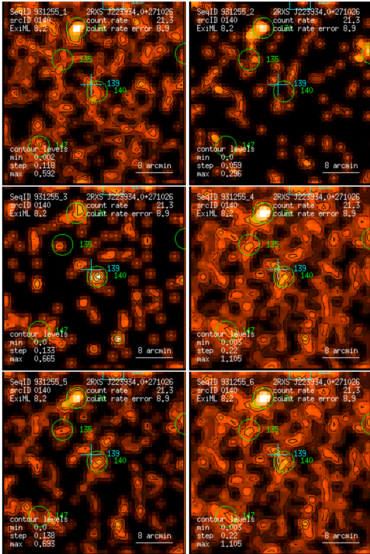
Figure 140: RASS 931255: detection 0140: band rate images, Gaussian filter: (1) PSPC channels 11 – 41, (2) 52 – 90, (3) 91 – 201, (4) 11 – 235, (5) 52 – 201, (6) 11 – 201. Broad band rates in counts/ks. Band rate contour levels in counts/ks/arcmin 2 .
