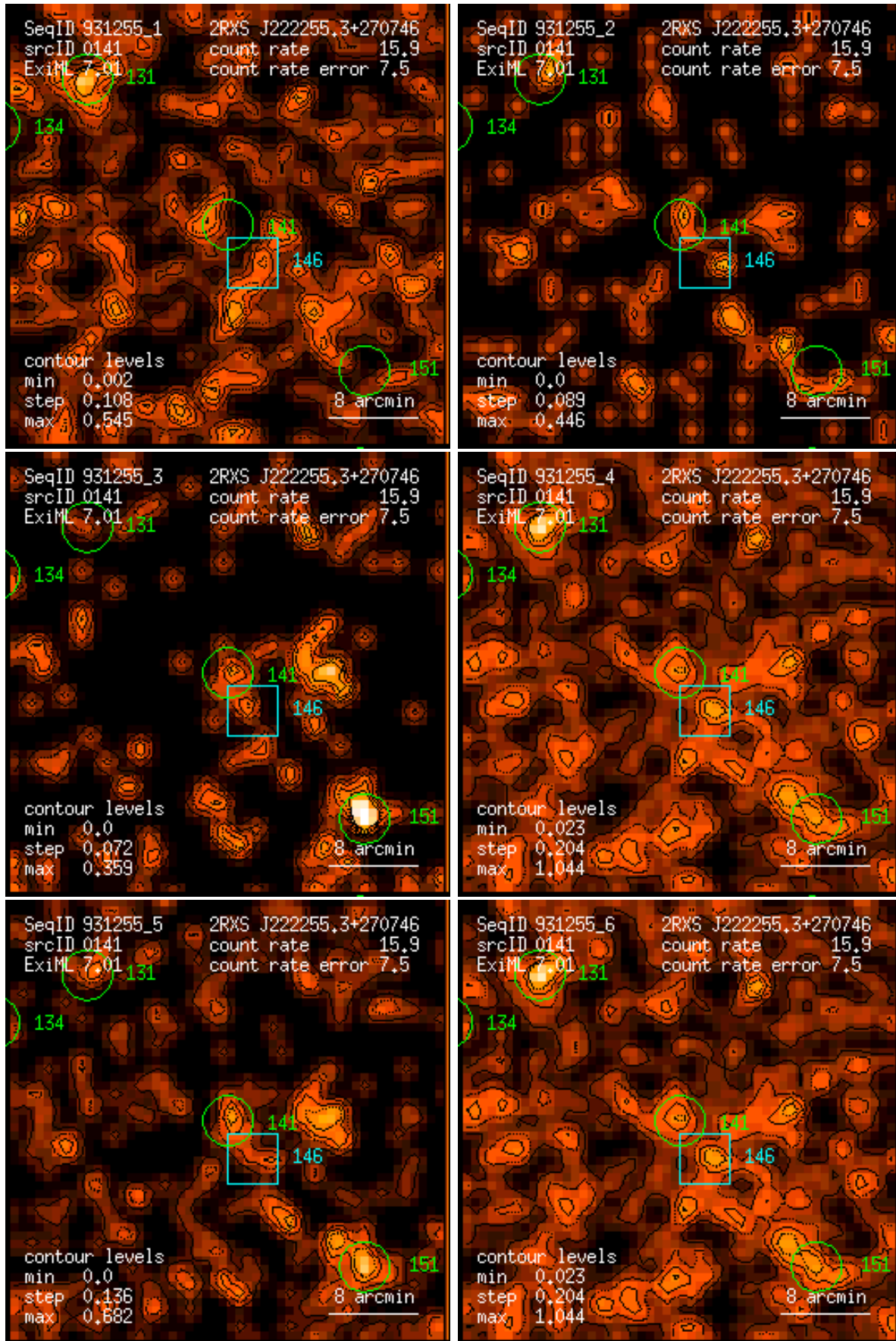
Figure 141: RASS 931255: detection 0141: band rate images, Gaussian filter: (1) PSPC channels 11 – 41, (2) 52 – 90, (3) 91 – 201, (4) 11 – 235, (5) 52 – 201, (6) 11 – 201. Broad band rates in counts/ks. Band rate contour levels in counts/ks/arcmin 2 .
